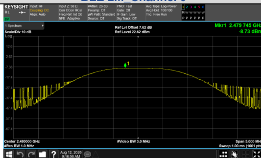
Peak Output Power BLE 1M_Channel 39
