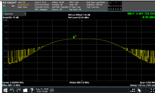
Peak Output Power BLE 1M_Channel 0
