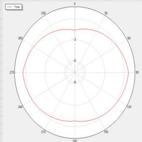
BLUETOOTH_Trp_H78 Total
