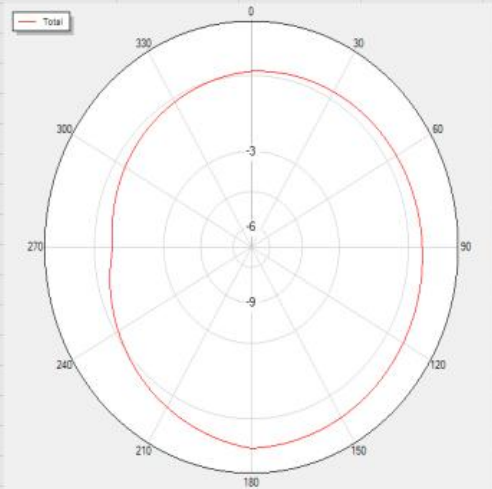
BLUETOOTH_Trp_H0 Total
