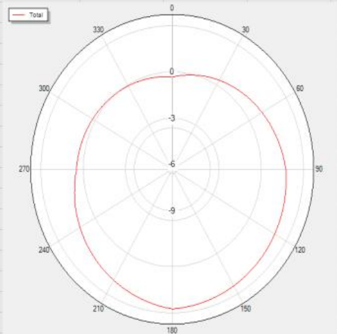
BLUETOOTH_Trp_H39 Total
