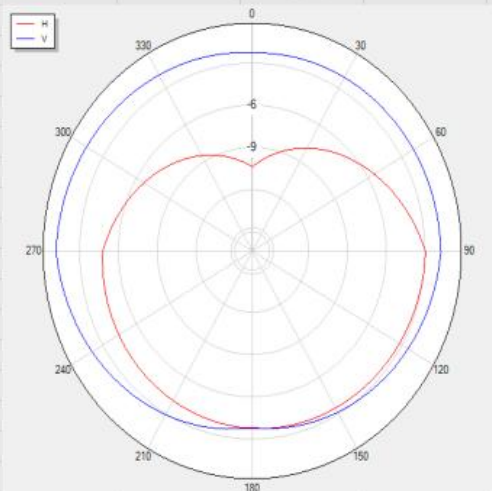
BLUETOOTH_Trp_H78 Polar
