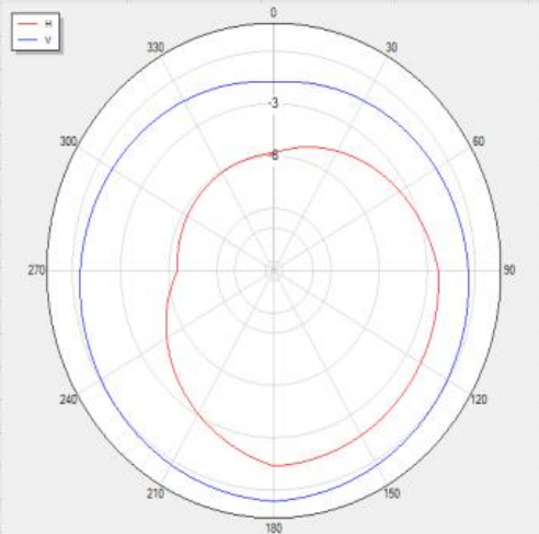
BLUETOOTH_Trp_H39 Polar
