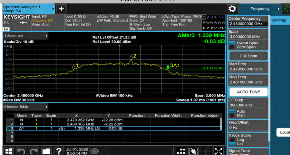
2DH5-Ant1-2480
