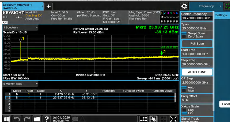
3DH5-Ant1-2480-1000~26500-PASS
