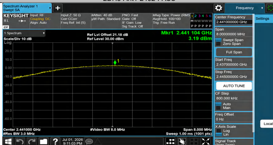
2DH5-Ant1-2441-PASS
