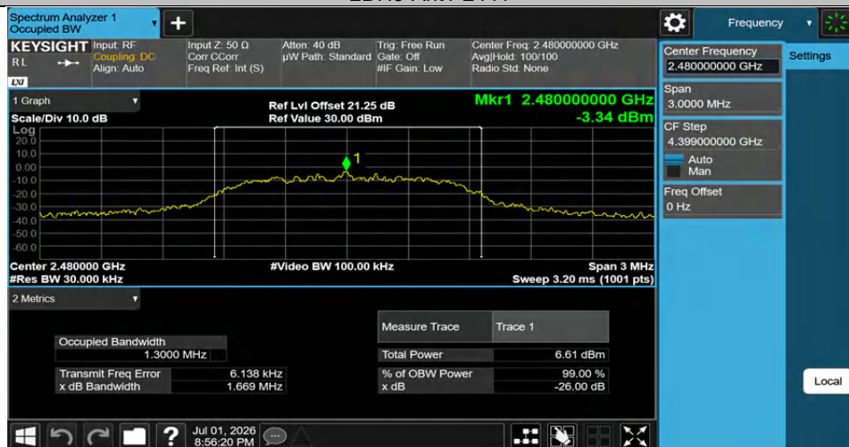
2DH5-Ant1-2480
