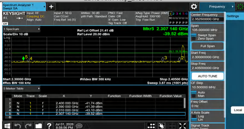
3DH5-Ant1-2402-PASS
