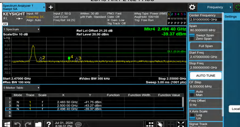
2DH5-Ant1-2480-PASS
