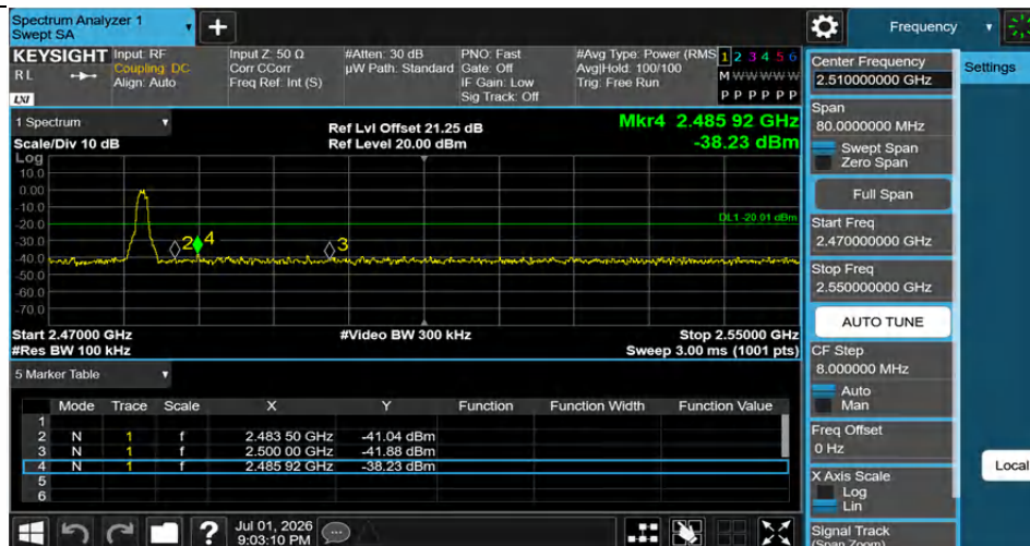
3DH5-Ant1-2480-PASS
