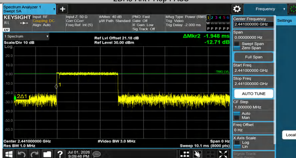
3DH5-Ant1-Hop-PASS
