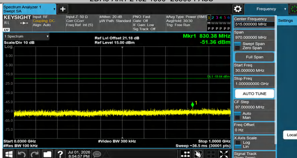
2DH5-Ant1-2441-30~1000-PASS
