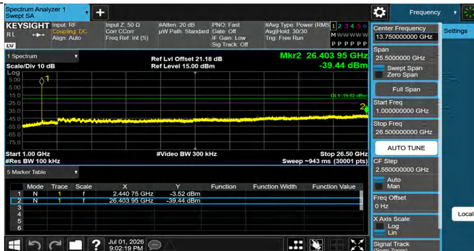
3DH5-Ant1-2441-1000~26500-PASS
