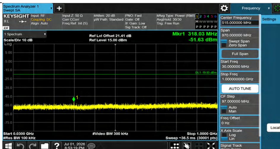
2DH5-Ant1-2402-30~1000-PASS
