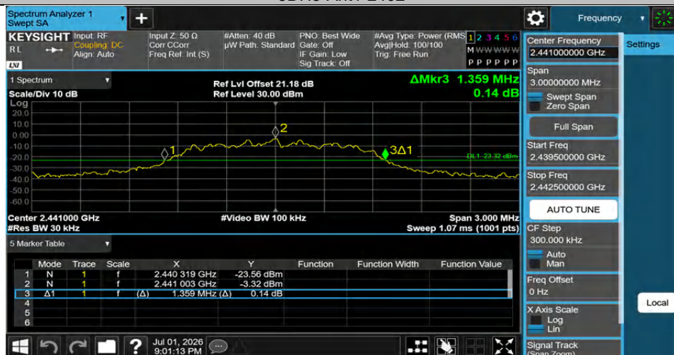
3DH5-Ant1-2441
