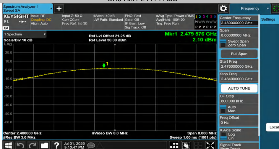
DH5-Ant1-2480-PASS
