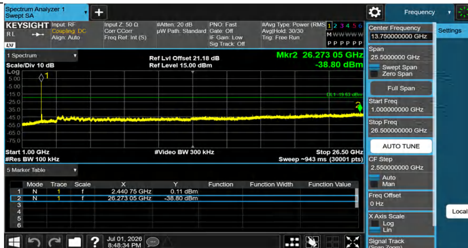
DH5-Ant1-2441-1000~26500-PASS
