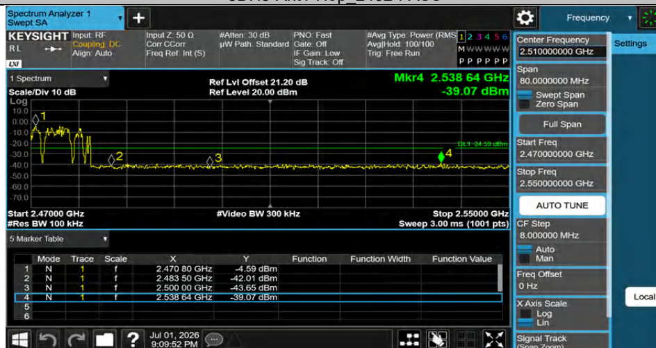
3DH5-Ant1-Hop_2480-PASS
