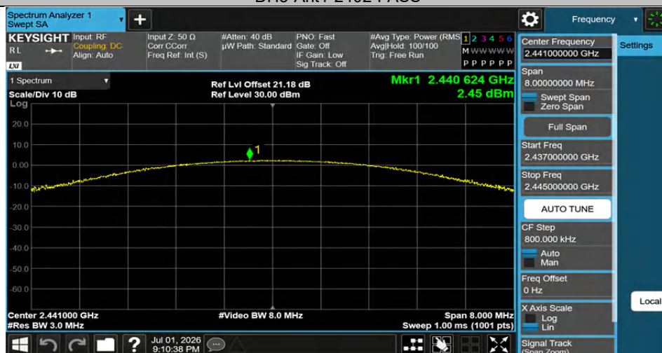
DH5-Ant1-2441-PASS
