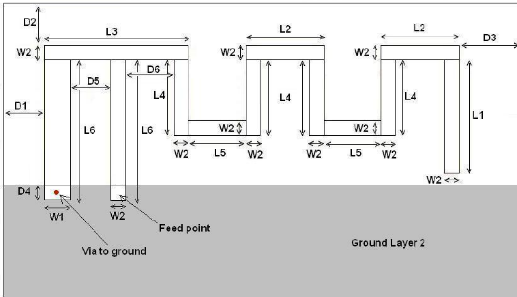
Figure 3: Antenna Dimensions
