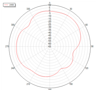
Theta=90 freq=2450MHz
