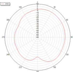
Phi=0 freq=2400MHz
