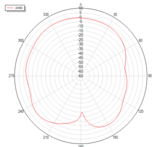
Phi=90 freq=2450MHz
