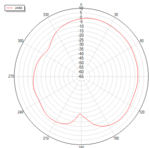
Phi=0 freq=2450MHz
