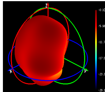
Phi=0 freq=2450MHz
