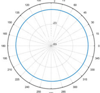
Total-Polar-H-640MHZ
