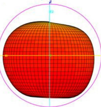
Total-3D-E1-640MHZ
