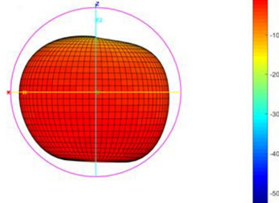
Total-3D-E1-690MHZ
