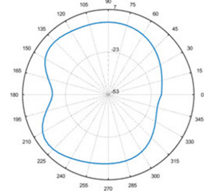
Total-Polar-E1-665MHZ
