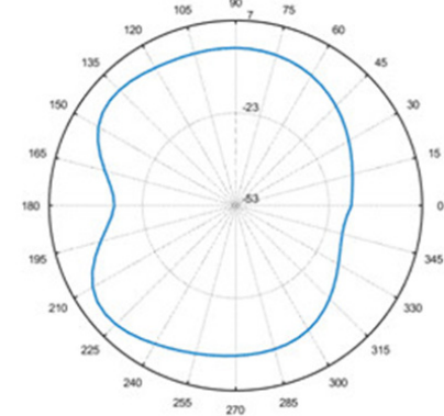
Total-Polar-E1-690MHZ
