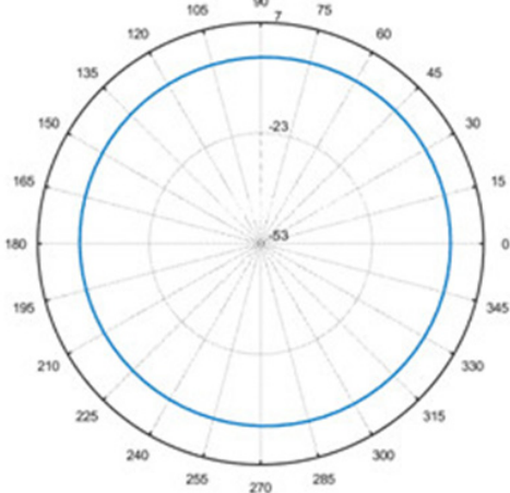
Total-Polar-H-665MHZ
