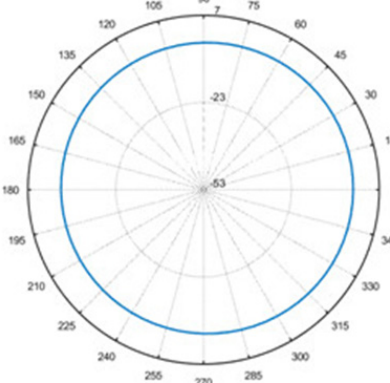
Total-Polar-E1-640MHZ
