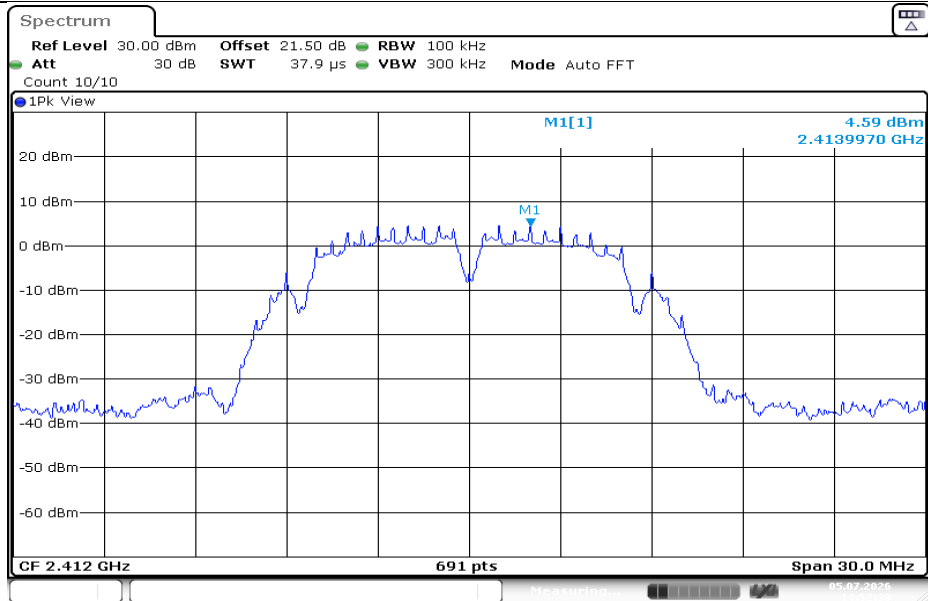
11B-Ant1-2412-0~Reference-PASS
