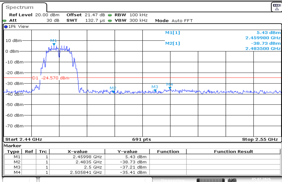
11B-Ant1-2462-PASS
