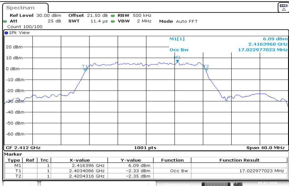
11G-Ant1-2412
