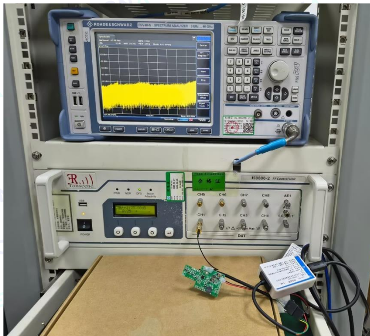
Photo of Setup for RF Conducted
