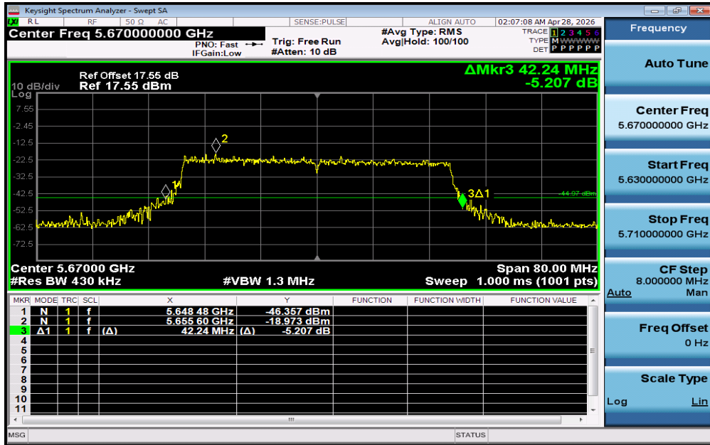
11AX40SISO-Ant1-5670
