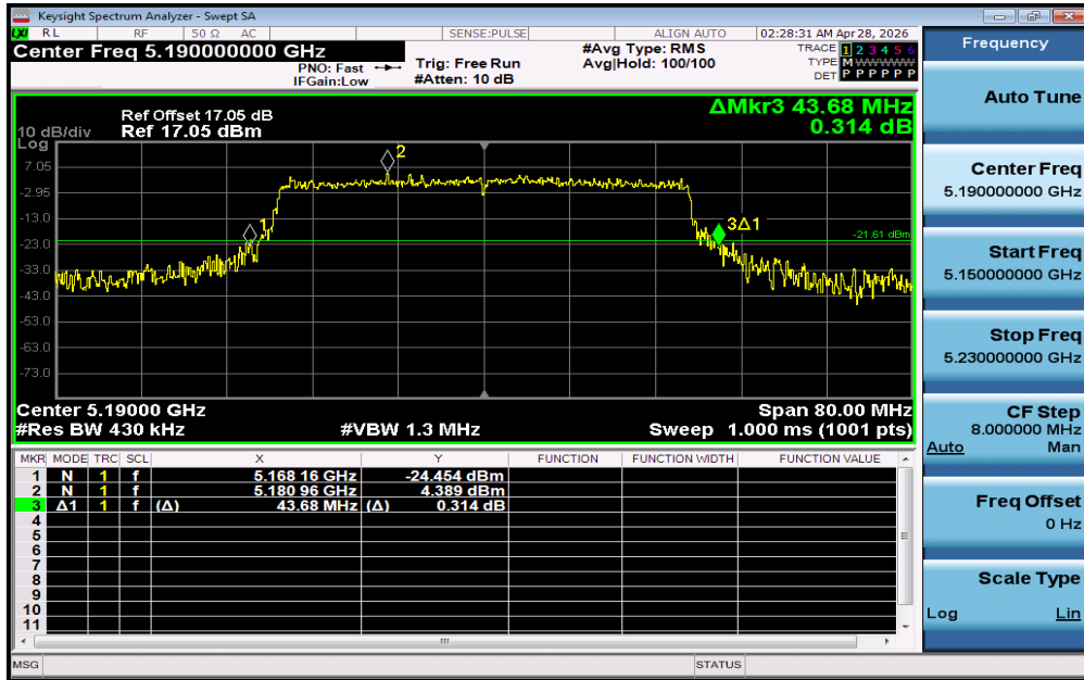
11AX40SISO-Ant1-5190
