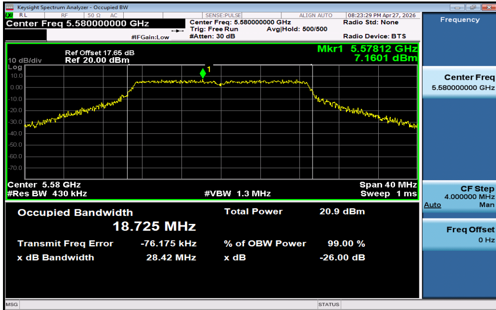
11AC20SISO-Ant1-5580
