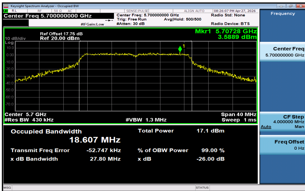
11AC20SISO-Ant1-5700
