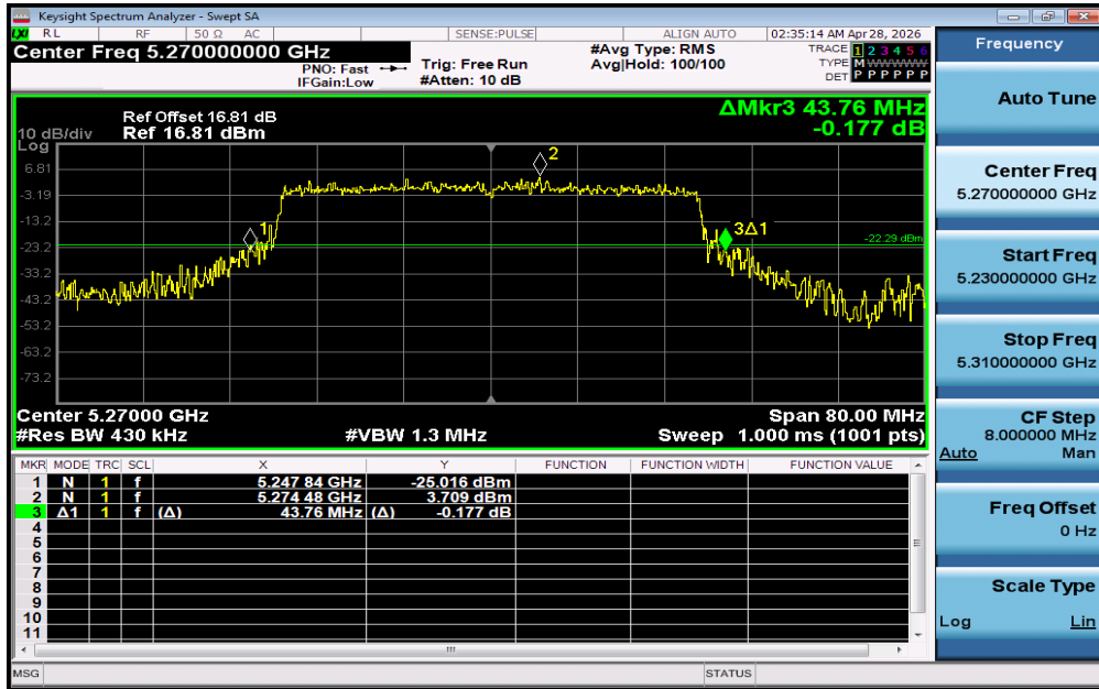
11AX40SISO-Ant1-5270
