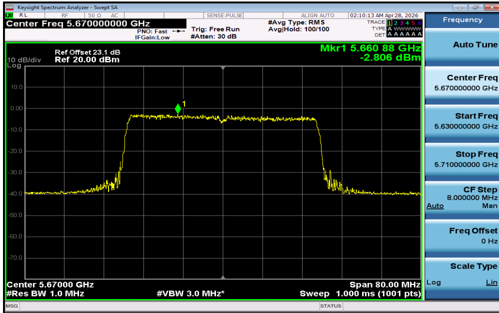
11AX40SISO-Ant1-5670-PASS
