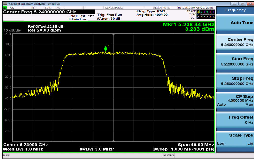
11AX20SISO-Ant1-5240-PASS
