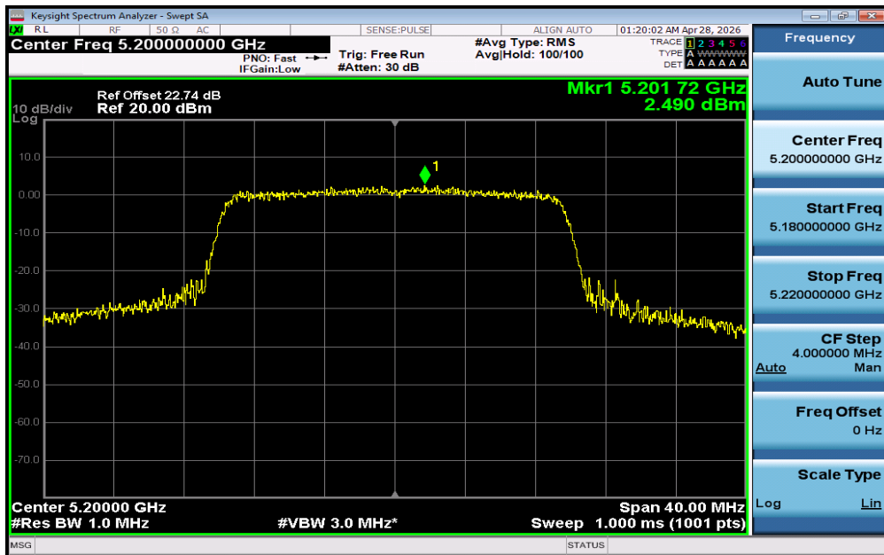
11AX20SISO-Ant1-5200-PASS
