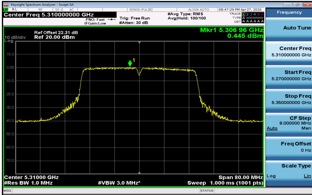
11AC40SISO-Ant1-5310-PASS
