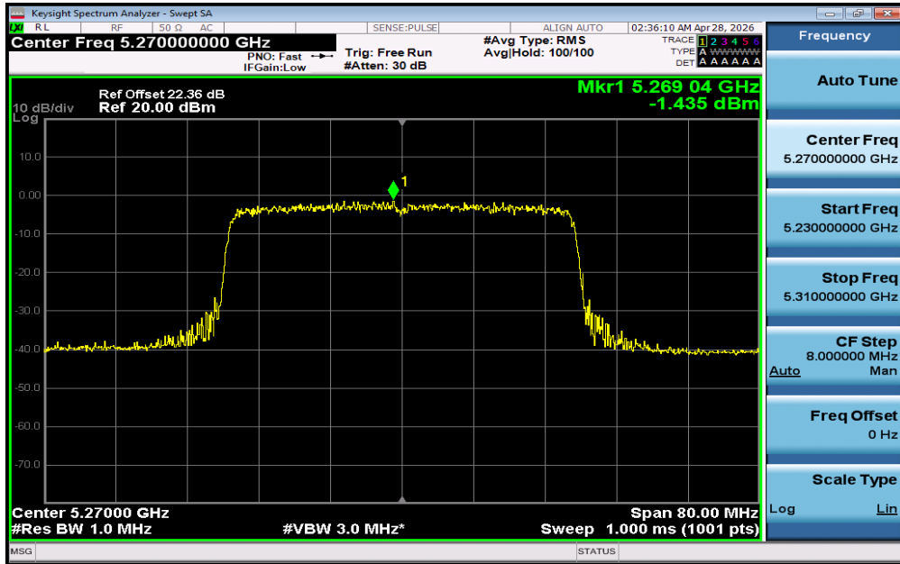
11AX40SISO-Ant1-5270-PASS
