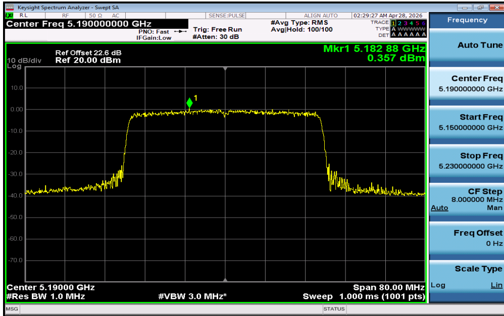
11AX40SISO-Ant1-5190-PASS
