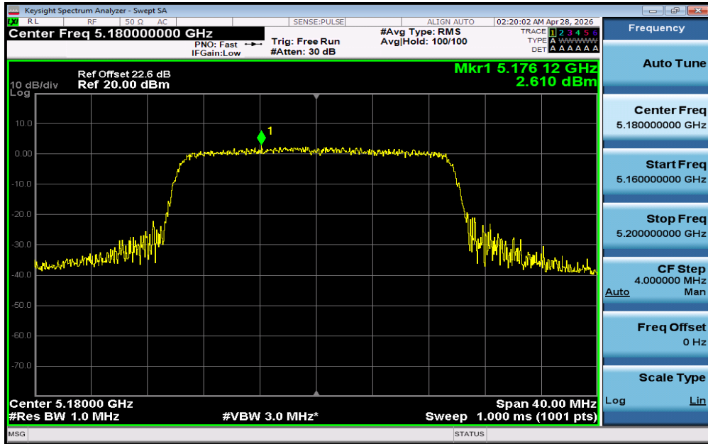
11AX20SISO-Ant1-5180-PASS
