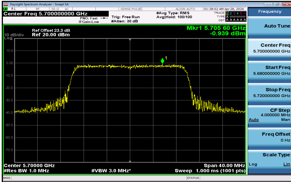
11AX20SISO-Ant1-5700-PASS
