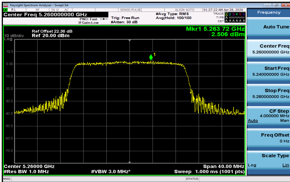
11AX20SISO-Ant1-5260-PASS
