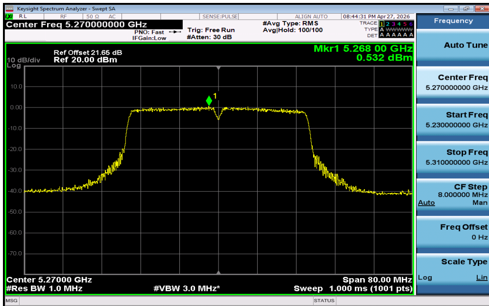
11AC40SISO-Ant1-5270-PASS
