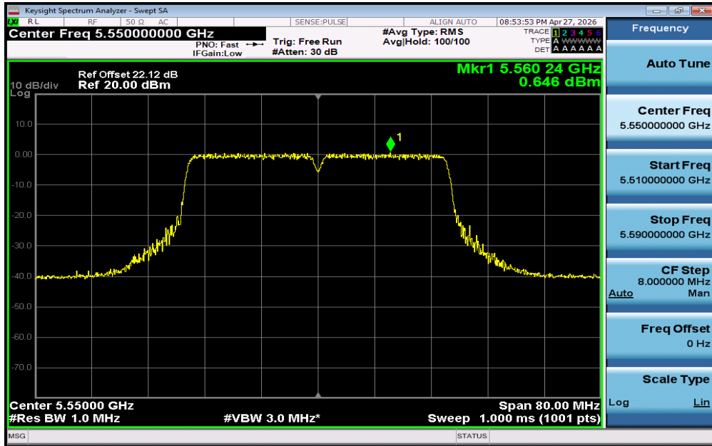
11AC40SISO-Ant1-5550-PASS
