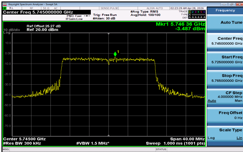
11AX20SISO-Ant1-5745-PASS
