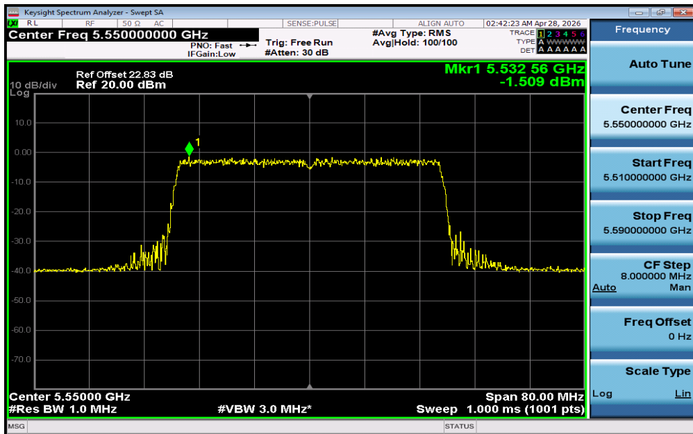
11AX40SISO-Ant1-5550-PASS
