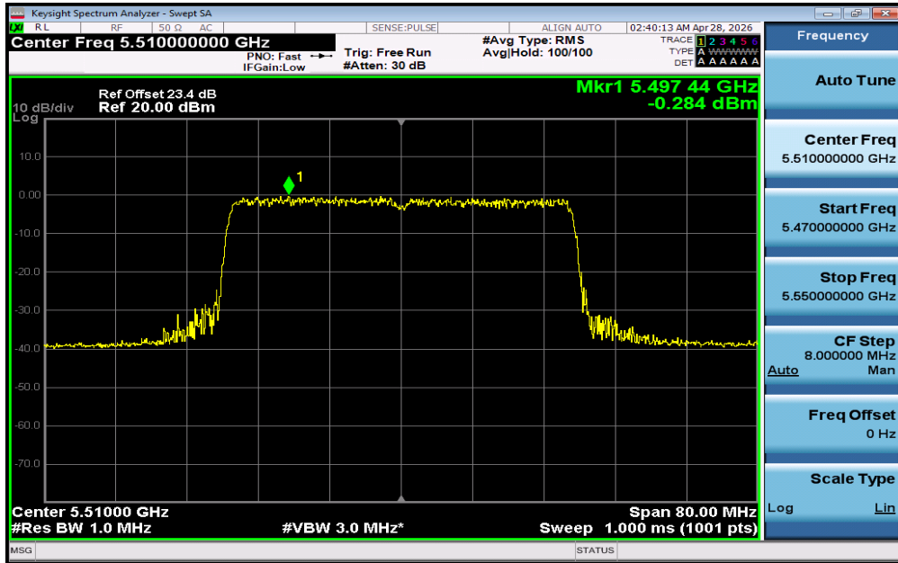
11AX40SISO-Ant1-5510-PASS
