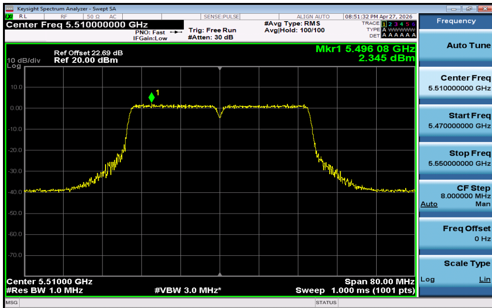
11AC40SISO-Ant1-5510-PASS
