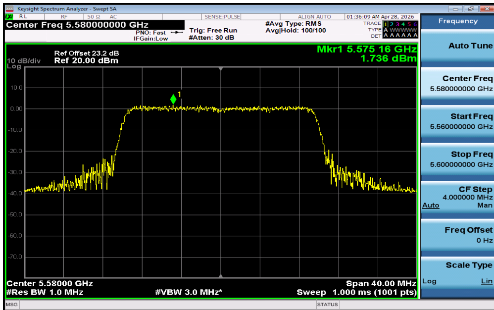
11AX20SISO-Ant1-5580-PASS
