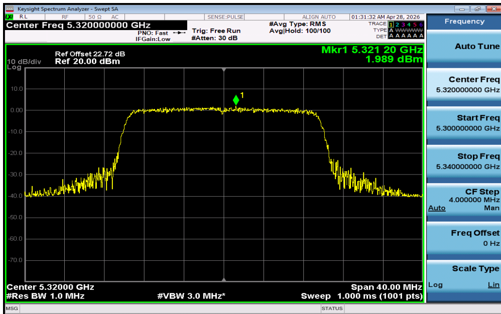
11AX20SISO-Ant1-5320-PASS
