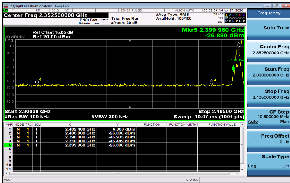
BLE_2M-Ant1-2402-PASS
