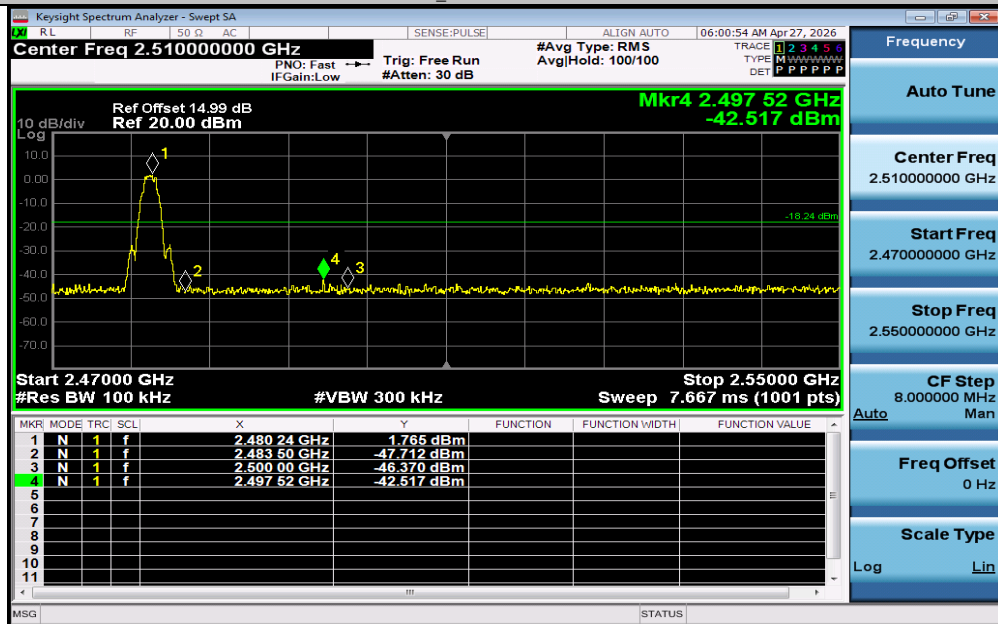
BLE_2M-Ant1-2480-PASS
