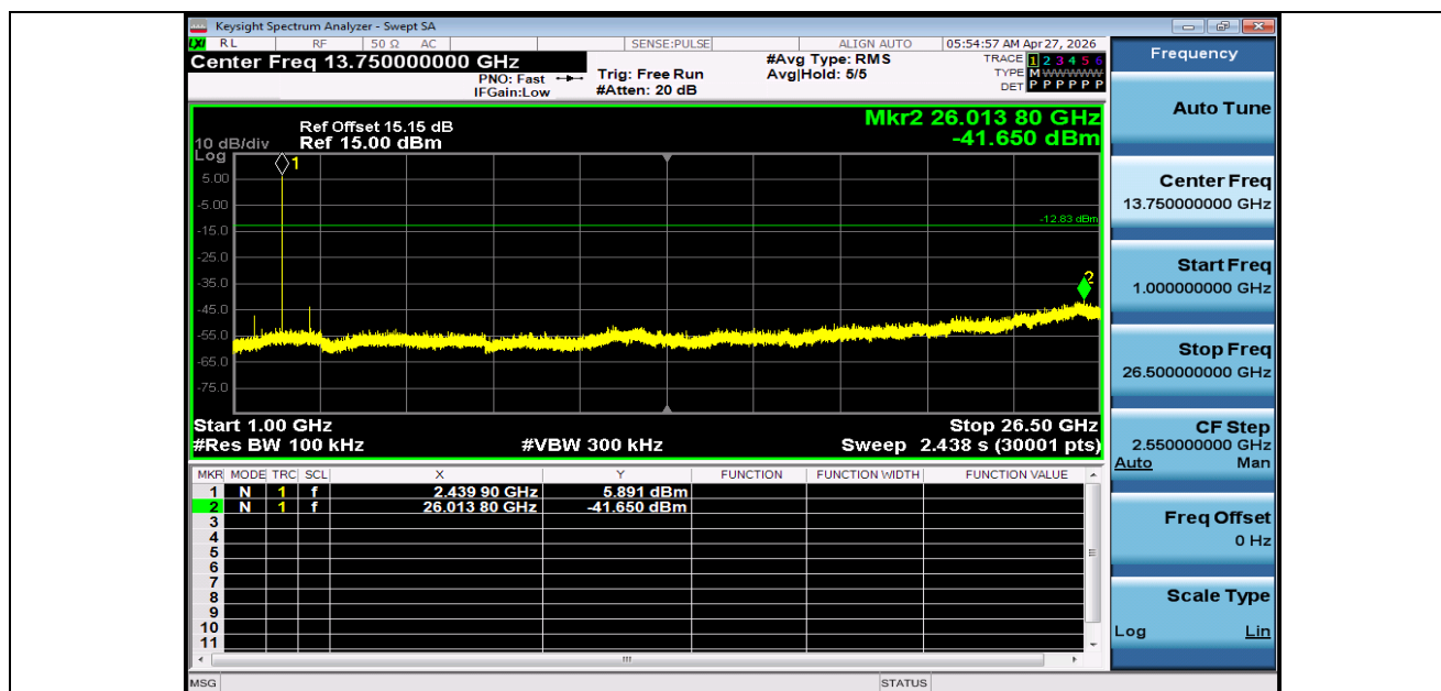
BLE_2M-Ant1-2440-1000-26500-PASS
