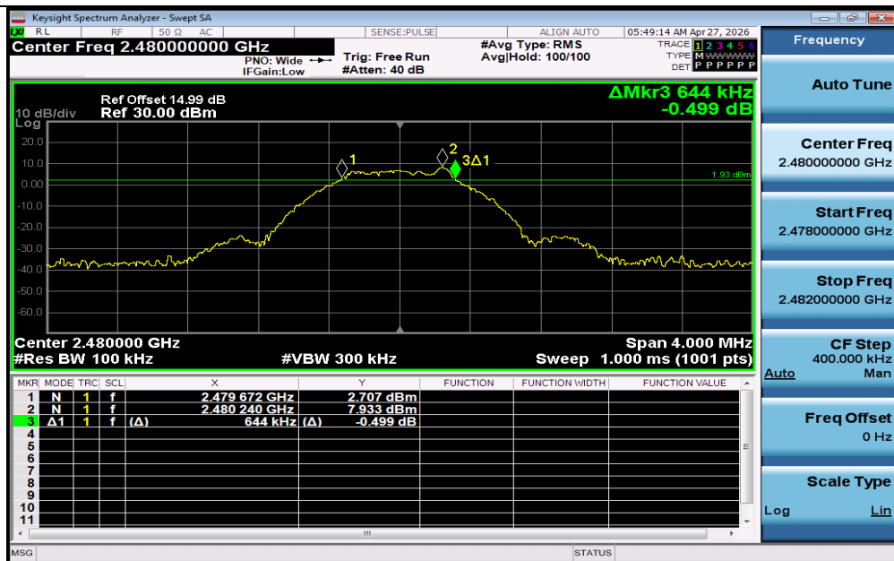
BLE_1M-Ant1-2480-PASS
