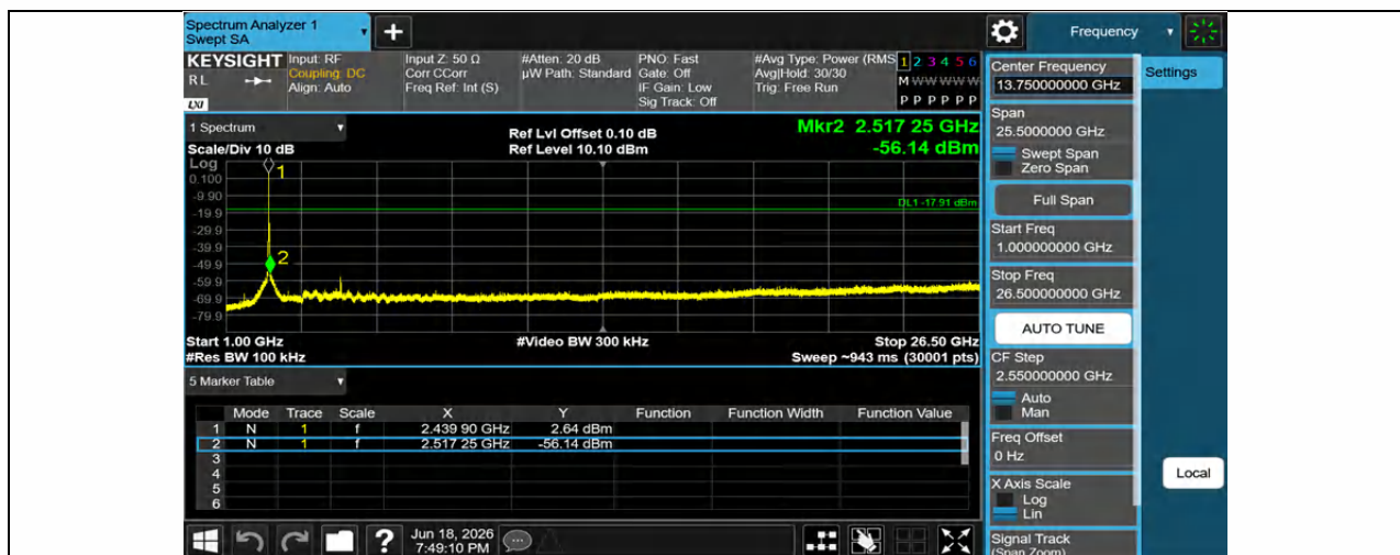
11N20SISO-Ant1-2437-1000~26500-PASS
