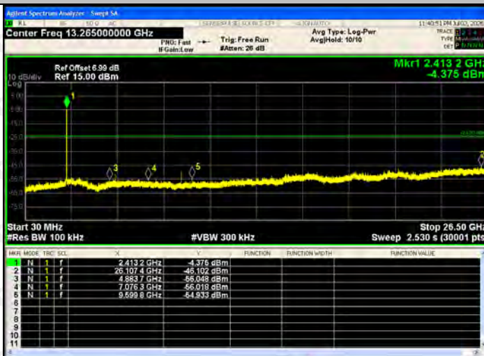
RF Conducted Spurious Emissions Graphs
