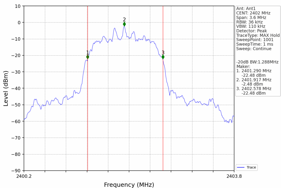
Pi/4DQPSK_2DH5_LCH_2402MHz_Ant1_NTV
