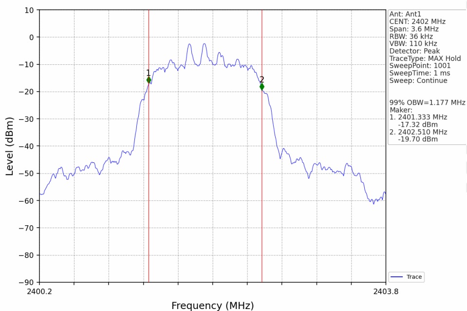
Pi/4DQPSK_2DH5_LCH_2402MHz_Ant1_NTNV
