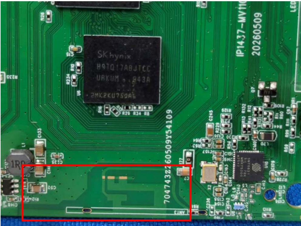
WIFI Antenna
