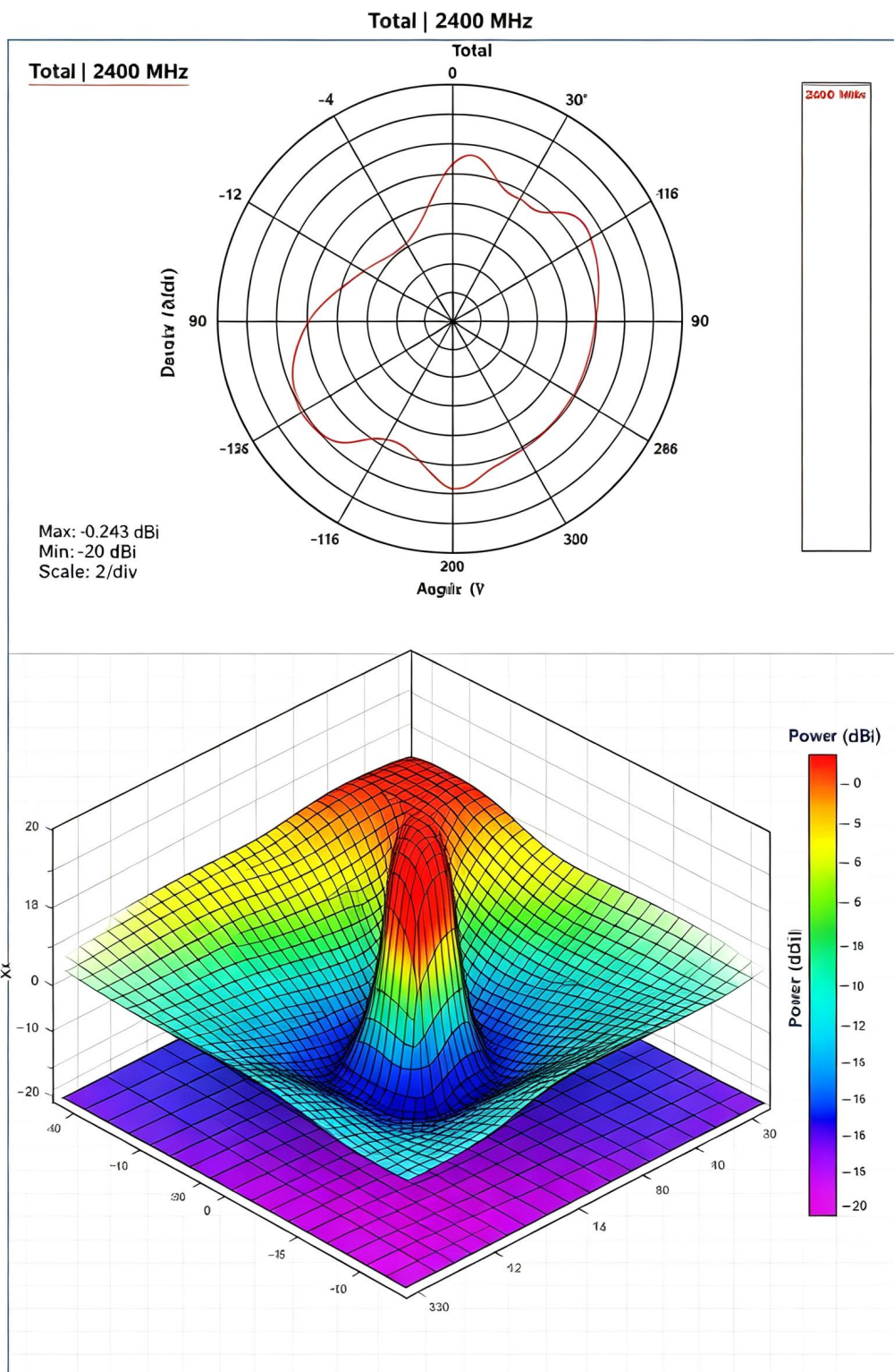
3-D Antenna Pattern Azimuth=0.0 Elevation=0.0 Roll=0.0
