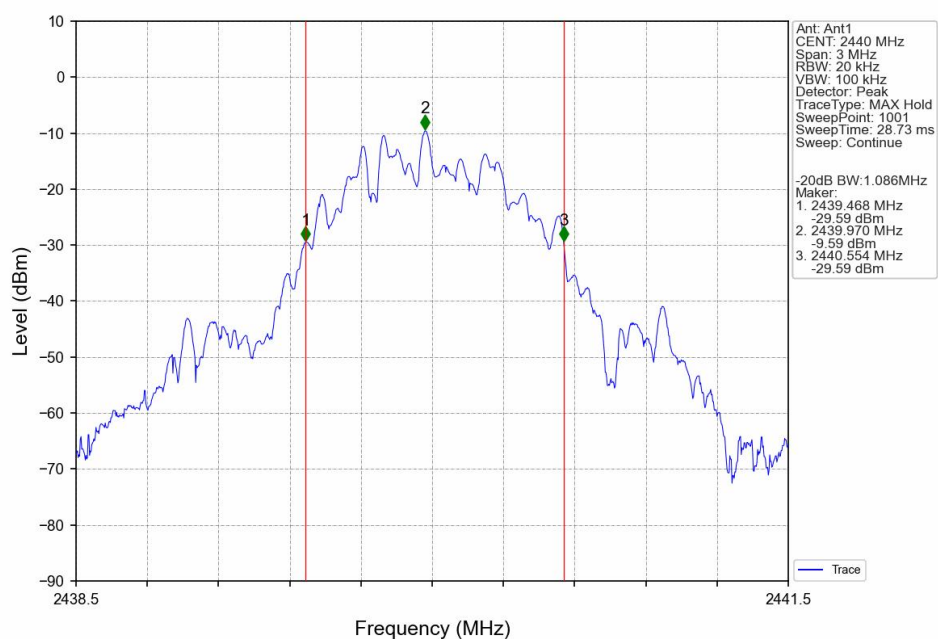
2.4G_MCH_2440MHz_Ant1_NTNV
