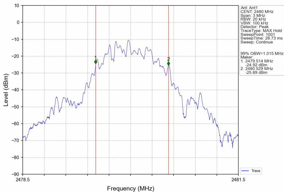
2.4G_HCH_2480MHz_Ant1_NTNV
