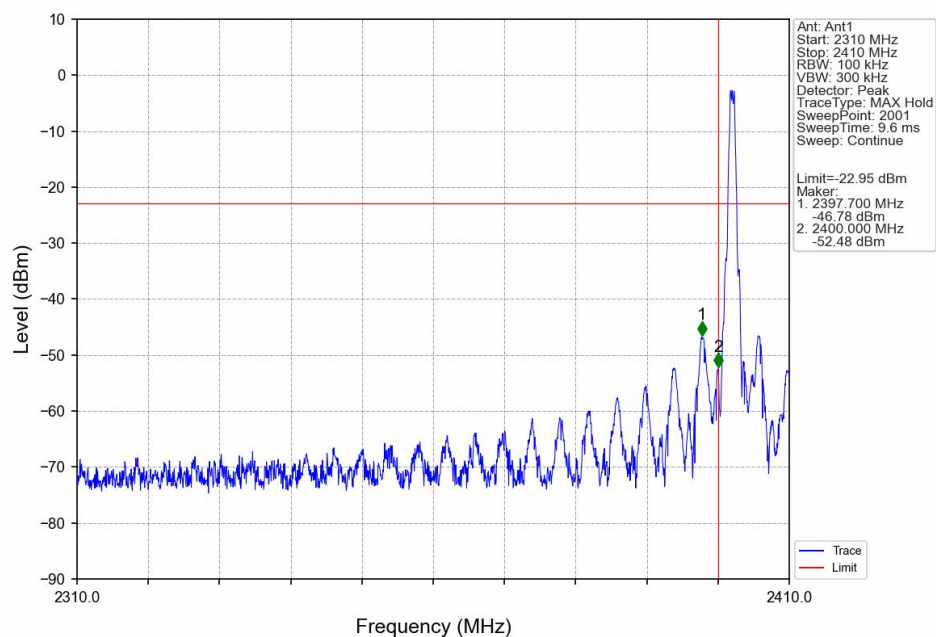
2.4G_LCH_2402MHz_Ant1_NTNV
