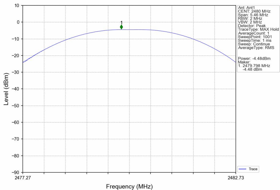
2.4G_HCH_2480MHz_Ant1_NTNV
