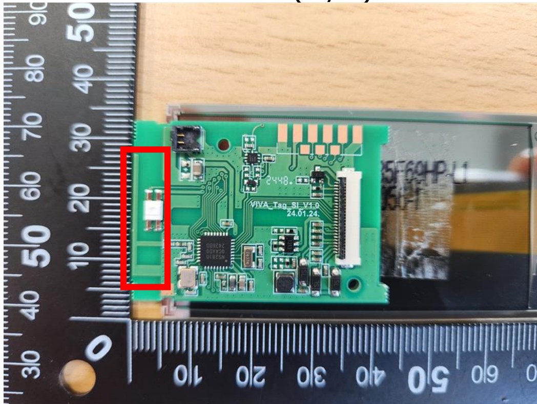
SRD Antenna(TX/RX)
