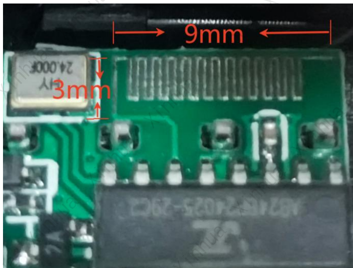
Antenna Dimensions
