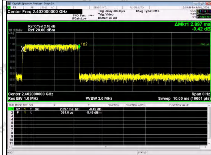
Dwell NVNT 3-DH5 2402MHz Ant1 Accumulated SISO
