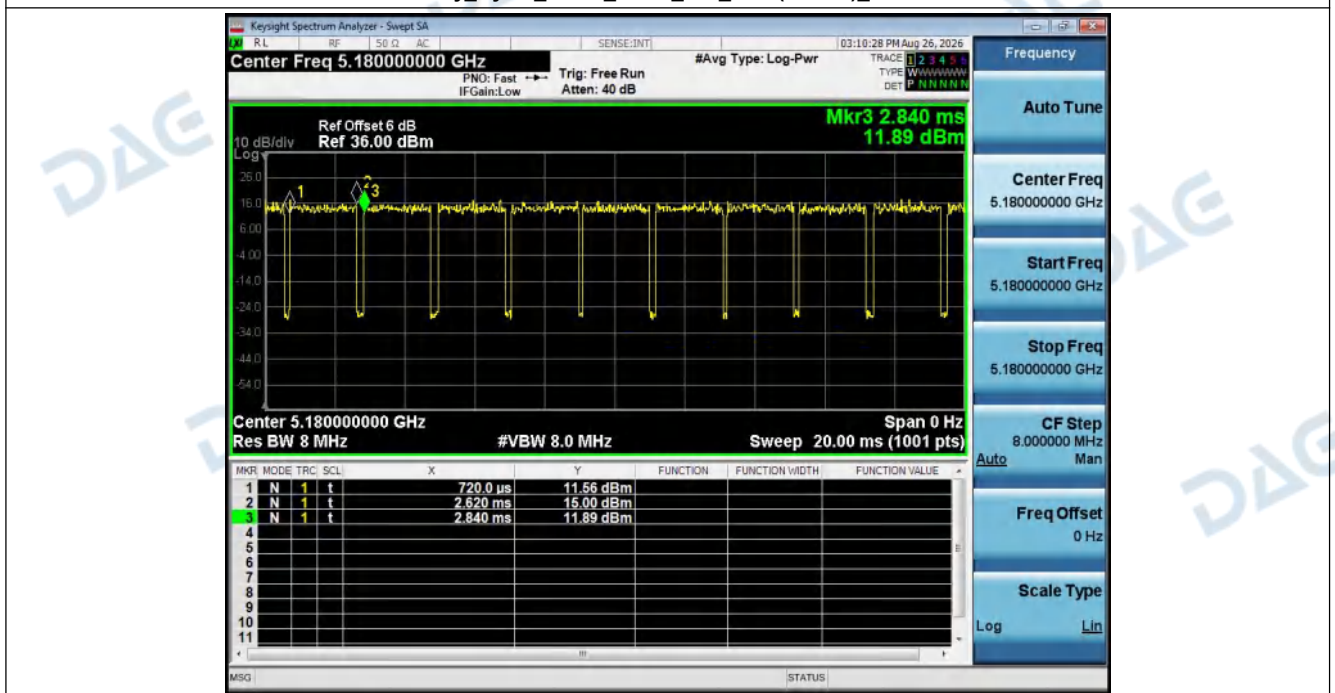
Duty_Cycle_NVNT_ANT1_802_11ac(VHT20)_5180
