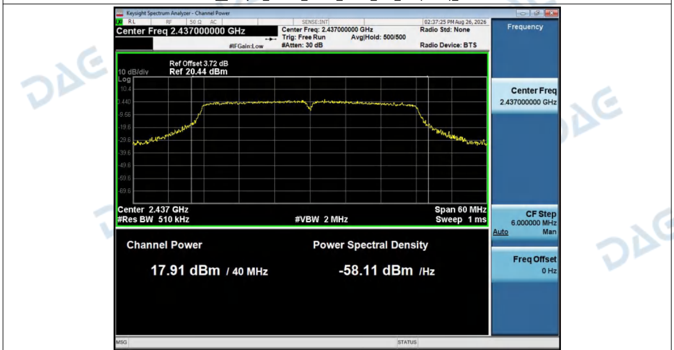
MAX__Output_Power_NVNT_ANT1_802_11n(HT40)_2437
