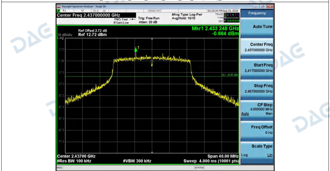
2_Spurious_Emission_NVNT_ANT1_802_11n(HT20)_2437
