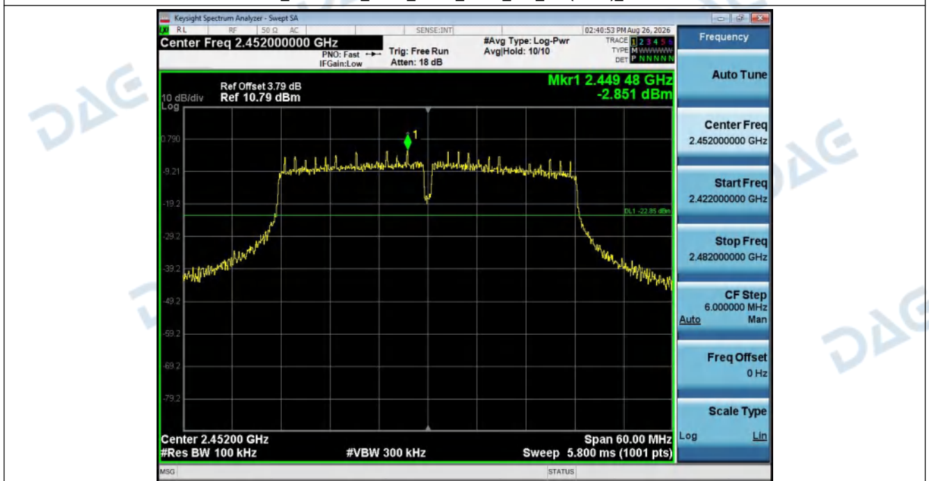
2_Bandedge_NVNT_ANT1_802_11n(HT40)_2452
