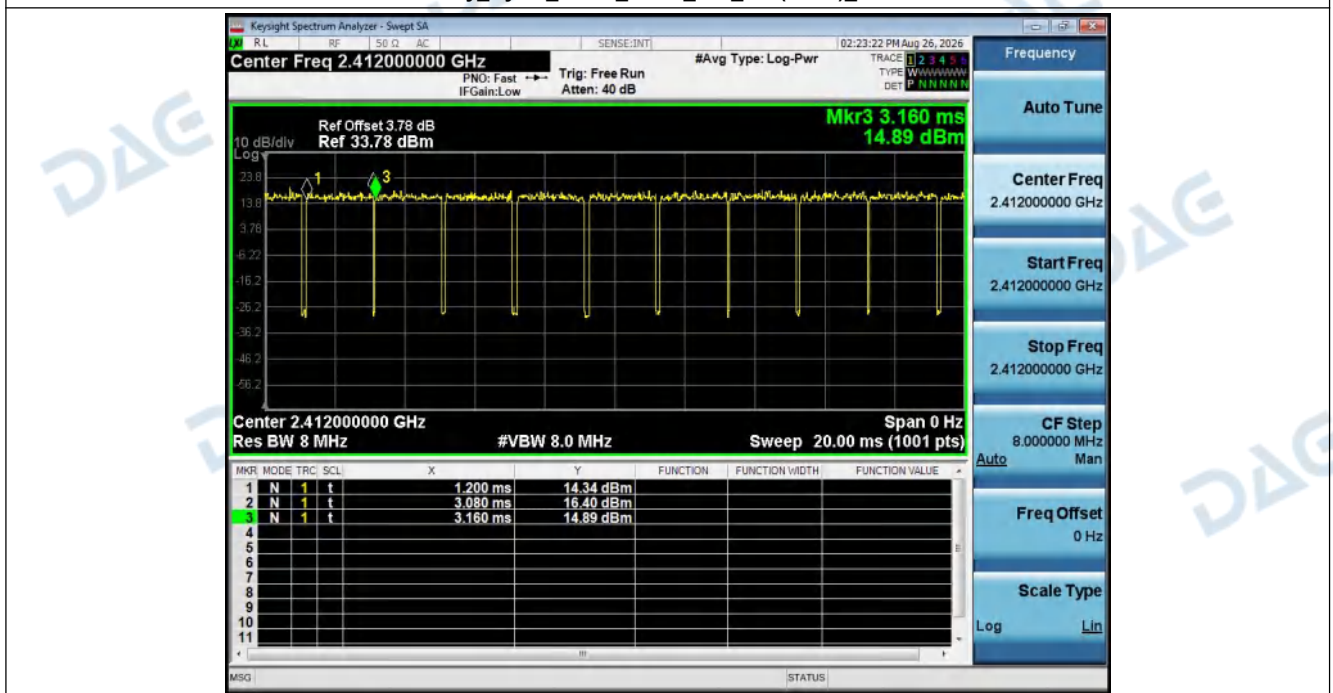
Duty_Cycle_NVNT_ANT1_802_11n(HT20)_2412
