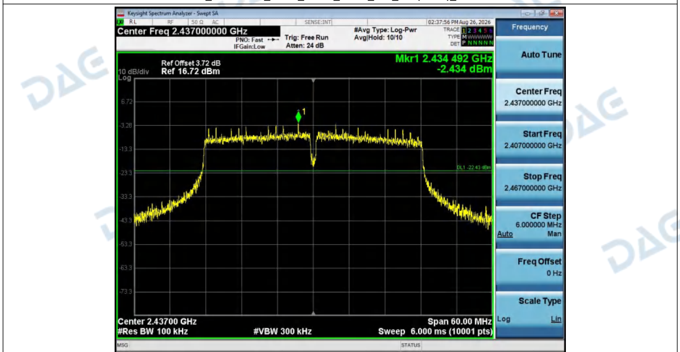
2_Spurious_Emission_NVNT_ANT1_802_11n(HT40)_2437
