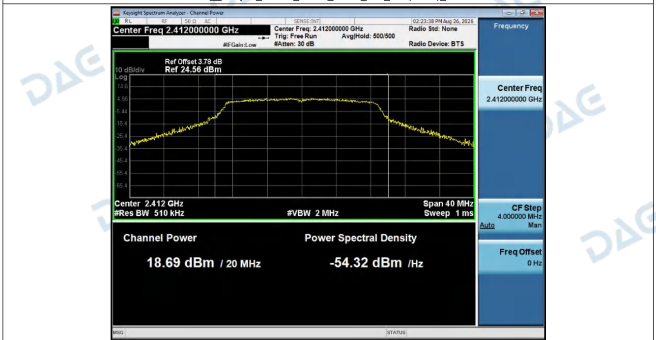
MAX__Output_Power_NVNT_ANT1_802_11n(HT20)_2412
