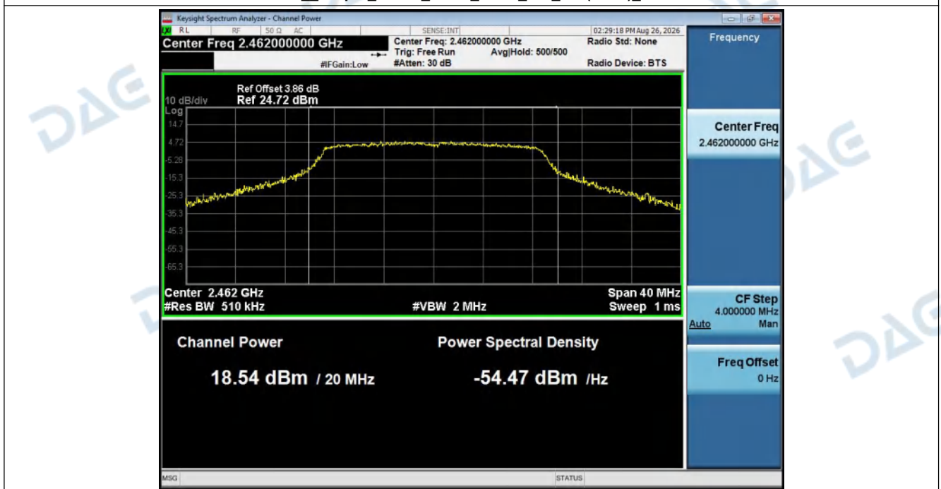
MAX__Output_Power_NVNT_ANT1_802_11n(HT20)_2462
