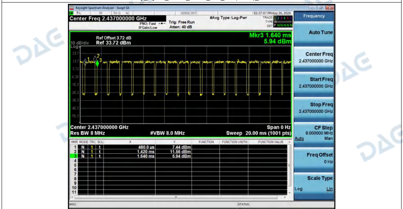
Duty_Cycle_NVNT_ANT1_802_11n(HT40)_2437
