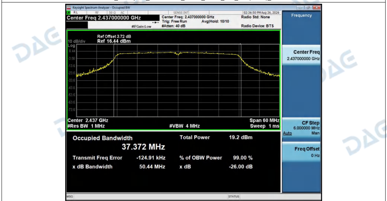
99%_Occupied_Bandwidth_NVNT_ANT1_802_11n(HT40)_2437
