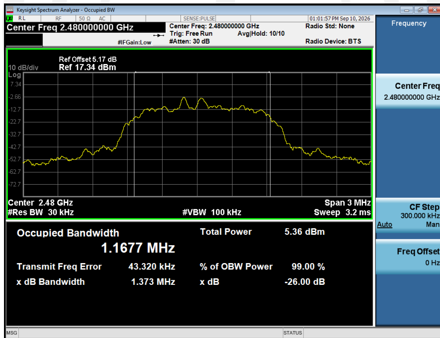
99%_Occupied_Bandwidth_NVNT_ANT1_2-DH1_2480_00
