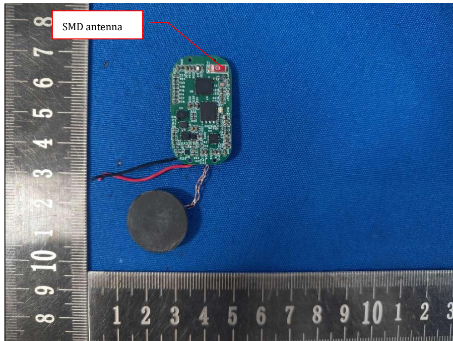
EUT Internal View 3
