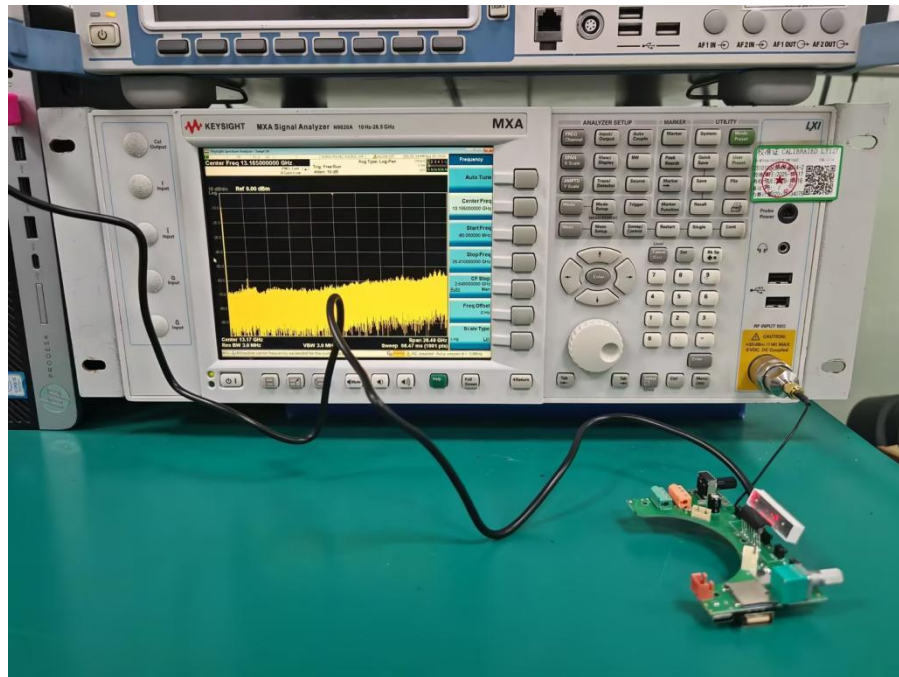
RF Conducted
