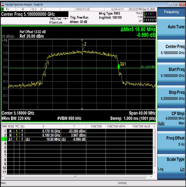
11AX20SISO-Ant1-5180
