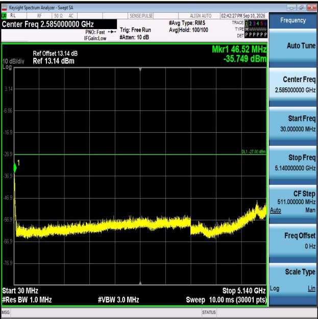
11AC20SISO-Ant1-5180-30~5140-PASS
