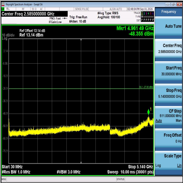
11AC20SISO-Ant1-5200-30~5140-PASS
