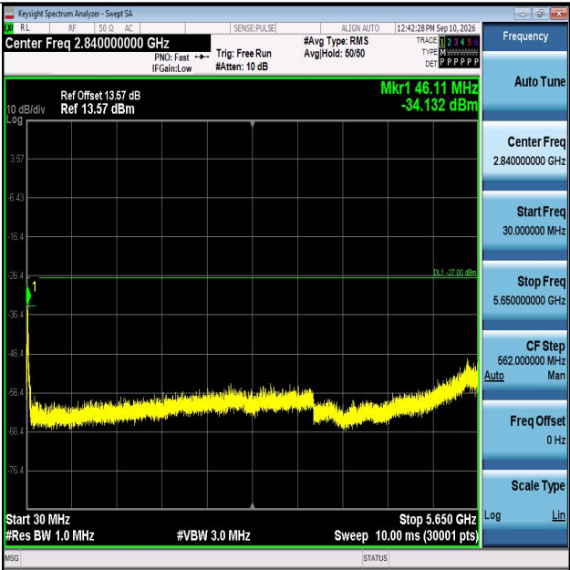
11N20SISO-Ant1-5745-30~5650-PASS
