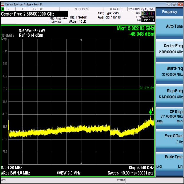
11AC20SISO-Ant1-5240-30~5140-PASS
