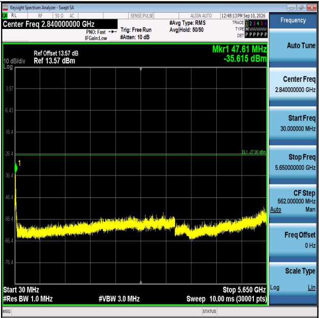
11N20SISO-Ant1-5785-30~5650-PASS
