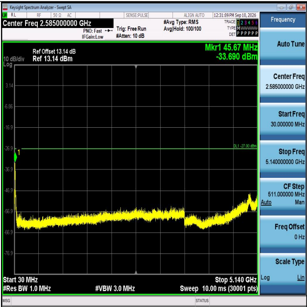
11N20SISO-Ant1-5200-30~5140-PASS
