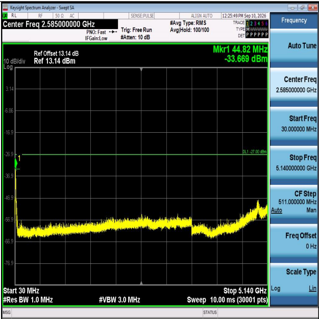
11N20SISO-Ant1-5180-30~5140-PASS
