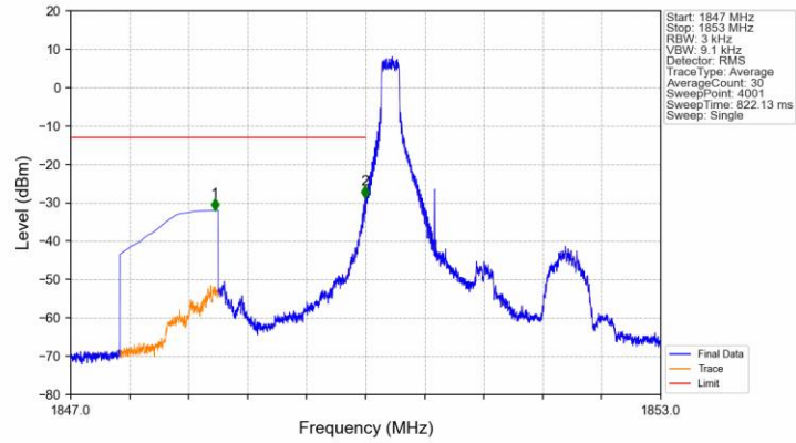
Band2_1.4MHz_QPSK_LCH_1850.7MHz_RB_1_0_NTNV
