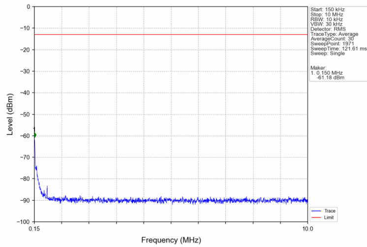
Band2_1.4MHz_QPSK_LCH_1850.7MHz_RB_1_0_NTNV
