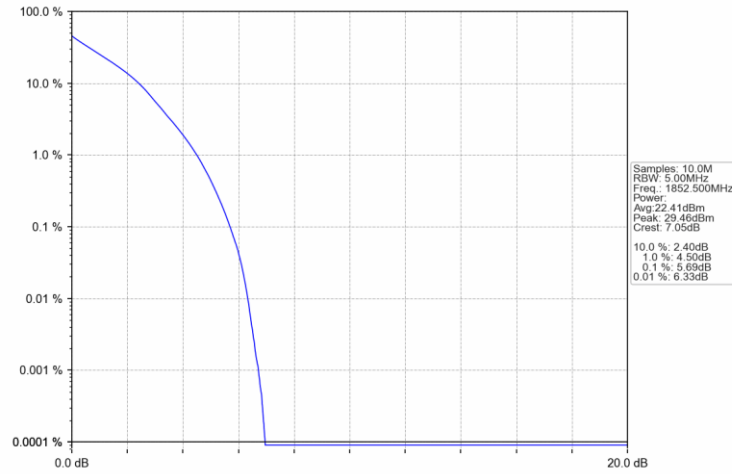
Band2_5MHz_QPSK_LCH_1852.5MHz_RB_25_0_NTNV
