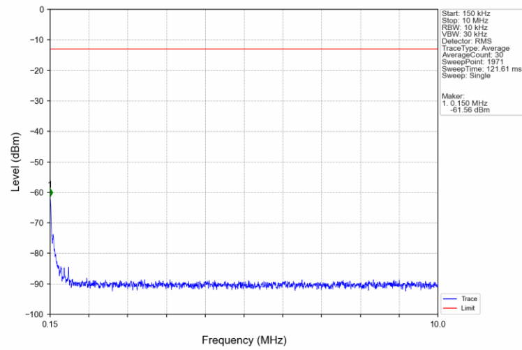
Band2_1.4MHz_16QAM_HCH_1909.3MHz_RB_1_0_NTNV
