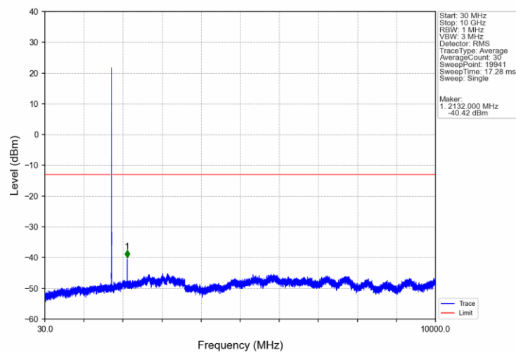
Band4_3MHz_16QAM_MCH_1732.5MHz_RB_1_0_NTNV
