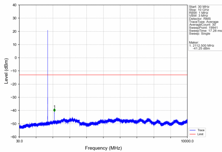
Band4_3MHz_16QAM_LCH_1711.5MHz_RB_1_0_NTNV
