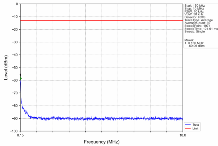
Band4_5MHz_QPSK_MCH_1732.5MHz_RB_1_0_NTNV
