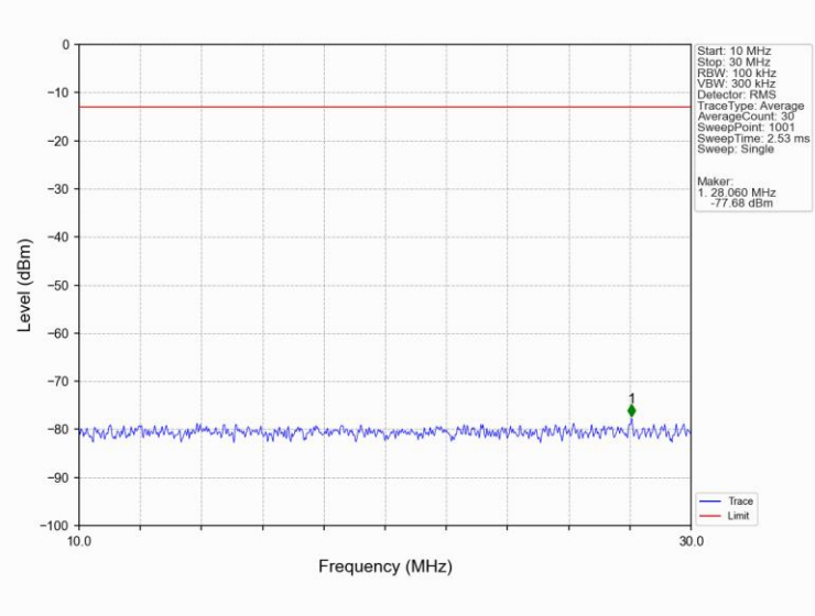
Band4_10MHz_16QAM_LCH_1715MHz_RB_1_0_NTNV
