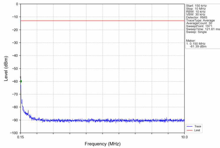
Band4_10MHz_16QAM_HCH_1750MHz_RB_1_0_NTNV
