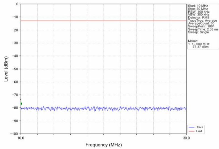
Band4_5MHz_16QAM_LCH_1712.5MHz_RB_1_0_NTNV
