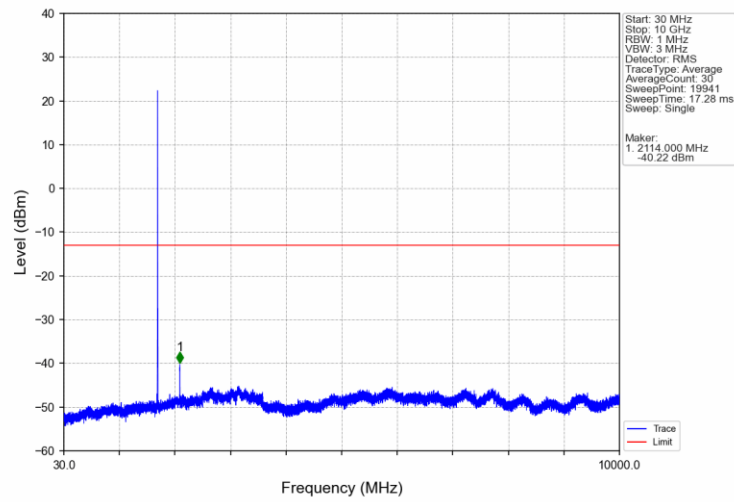
Band4_5MHz_QPSK_LCH_1712.5MHz_RB_1_0_NTNV
