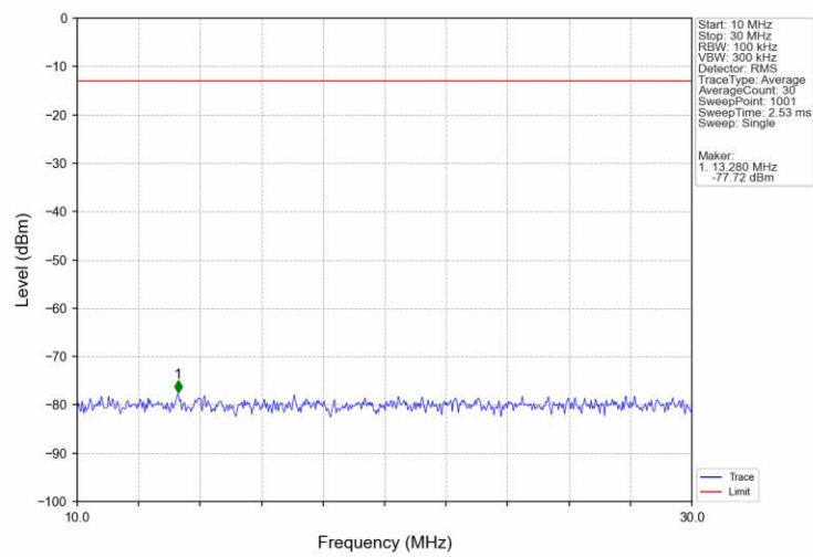
Band4_5MHz_QPSK_MCH_1732.5MHz_RB_1_0_NTNV
