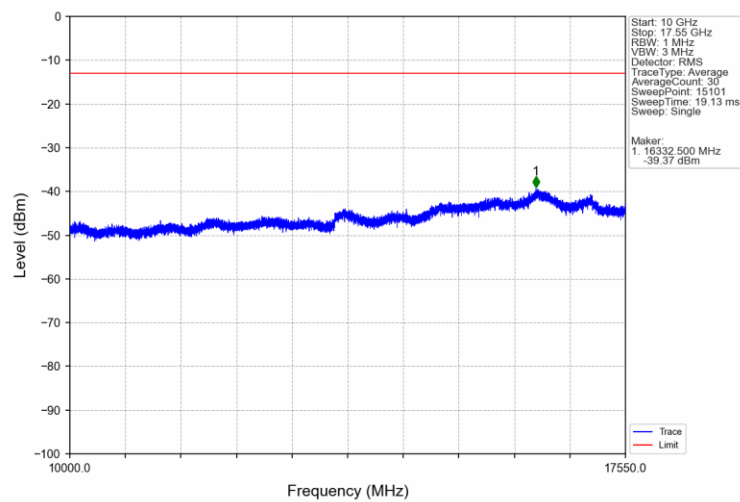
Band4_15MHz_QPSK_MCH_1732.5MHz_RB_1_0_NTNV
