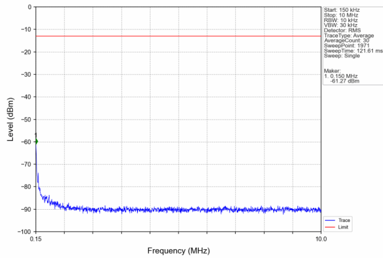
Band4_15MHz_QPSK_MCH_1732.5MHz_RB_1_0_NTNV
