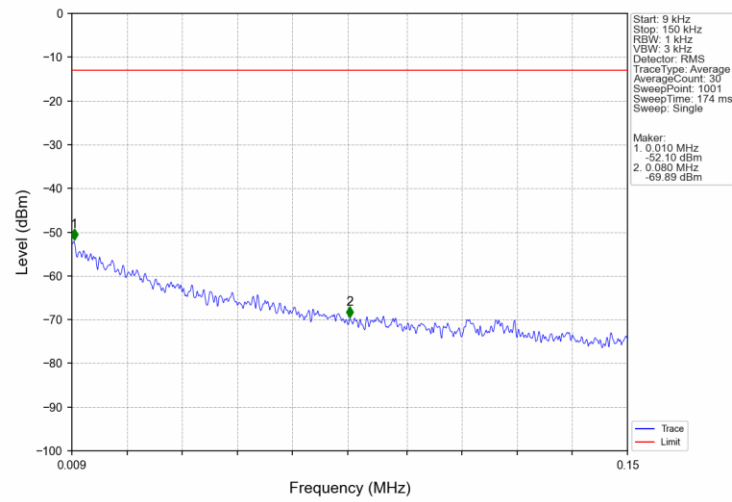
Band66_3MHz_16QAM_MCH_1745MHz_RB_1_0_NTNV
