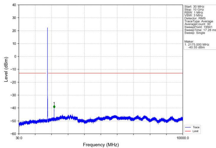
Band66_10MHz_QPSK_HCH_1775MHz_RB_1_0_NTNV
