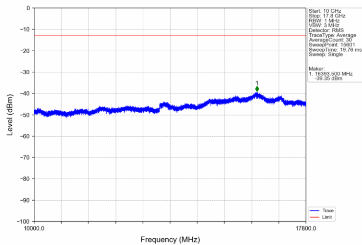
Band66_5MHz_QPSK_MCH_1745MHz_RB_1_0_NTNV
