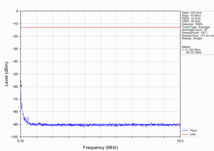
Band66_3MHz_16QAM_HCH_1778.5MHz_RB_1_0_NTNV
