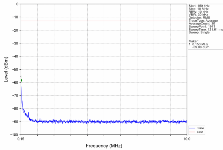
Band66_5MHz_QPSK_MCH_1745MHz_RB_1_0_NTNV
