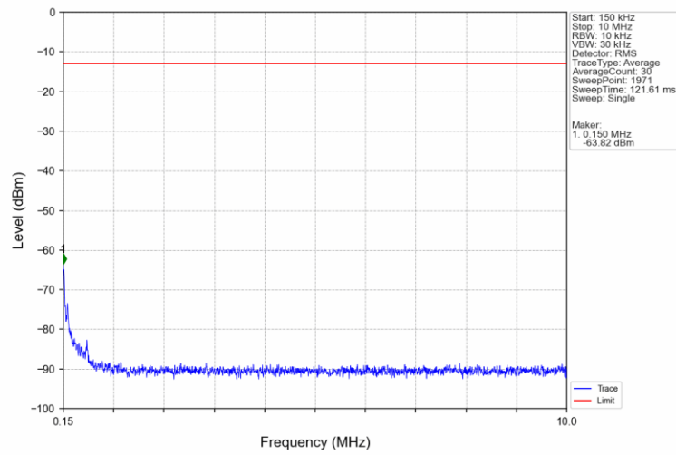
Band66_5MHz_16QAM_HCH_1777.5MHz_RB_1_0_NTNV
