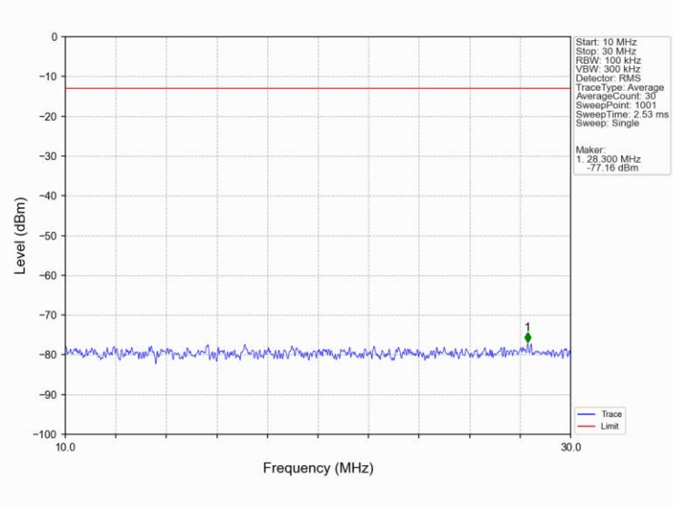
Band66_10MHz_QPSK_HCH_1775MHz_RB_1_0_NTNV
