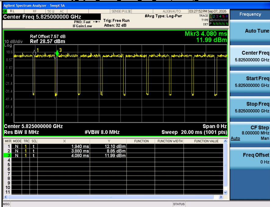
Duty Cycle NVNT ANT2_802_11ac(VHT20)_5825
