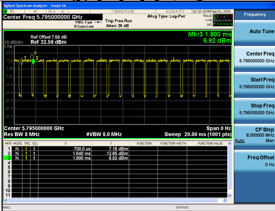
Duty_Cycle_NVNT_ANT1_802_11ac(VHT40)_5795
