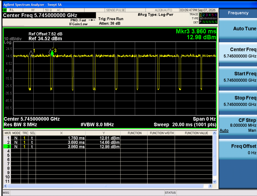
Duty_Cycle_NVNT_ANT2_802_11ac(VHT20)_5745
