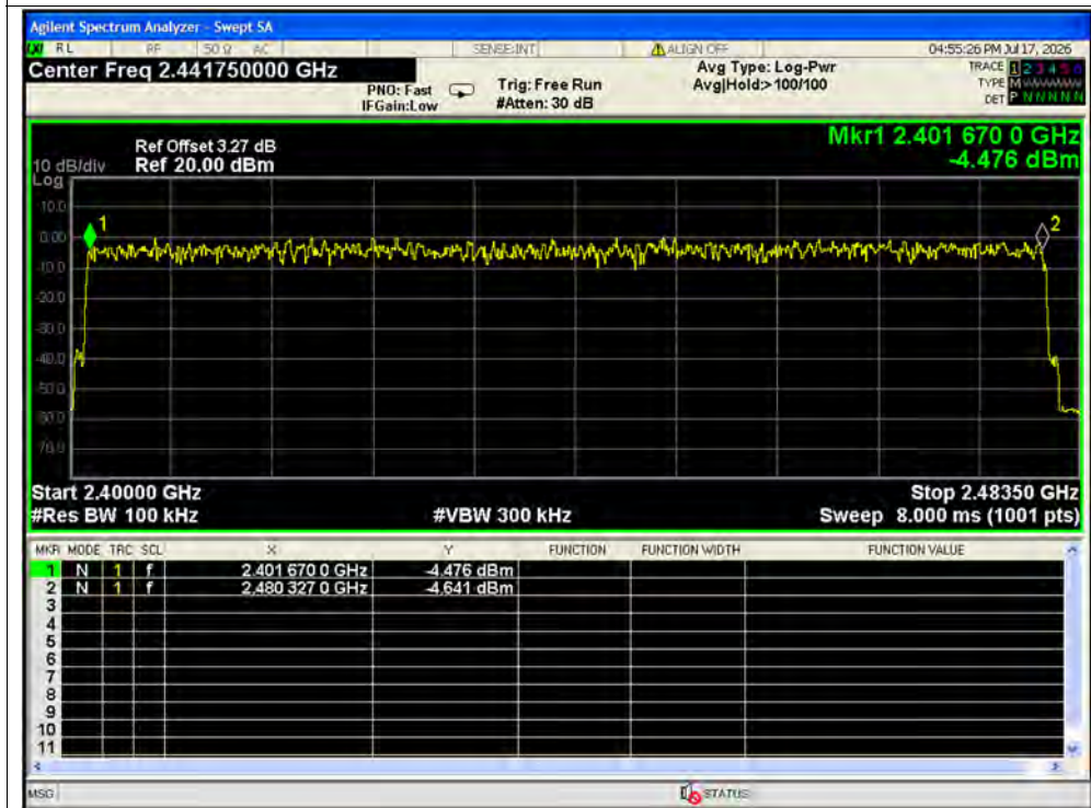
Hopping No. NVNT 2-DH5 2441MHz Ant1
