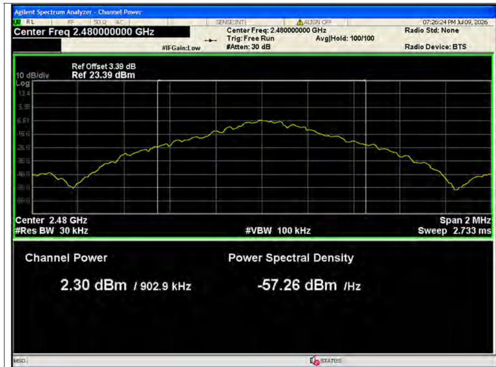
Average Power NVNT 1-DH5 2480MHz Ant1
