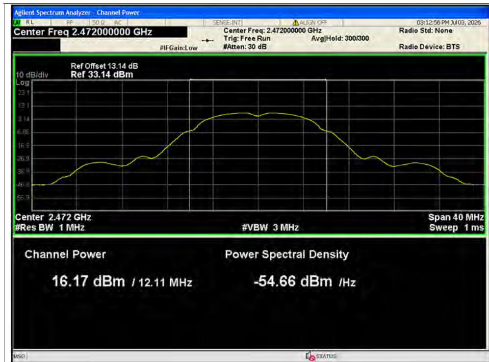
Average Power NVNT b 2472MHz Ant1
