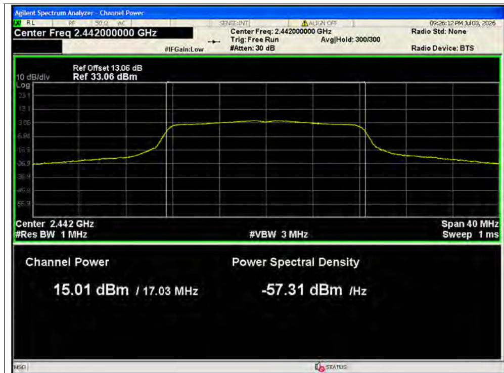
Average Power NVNT g 2442MHz Ant1
