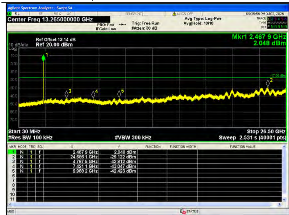
Tx. Spurious NVNT n20 2472MHz Ant1 Emission
