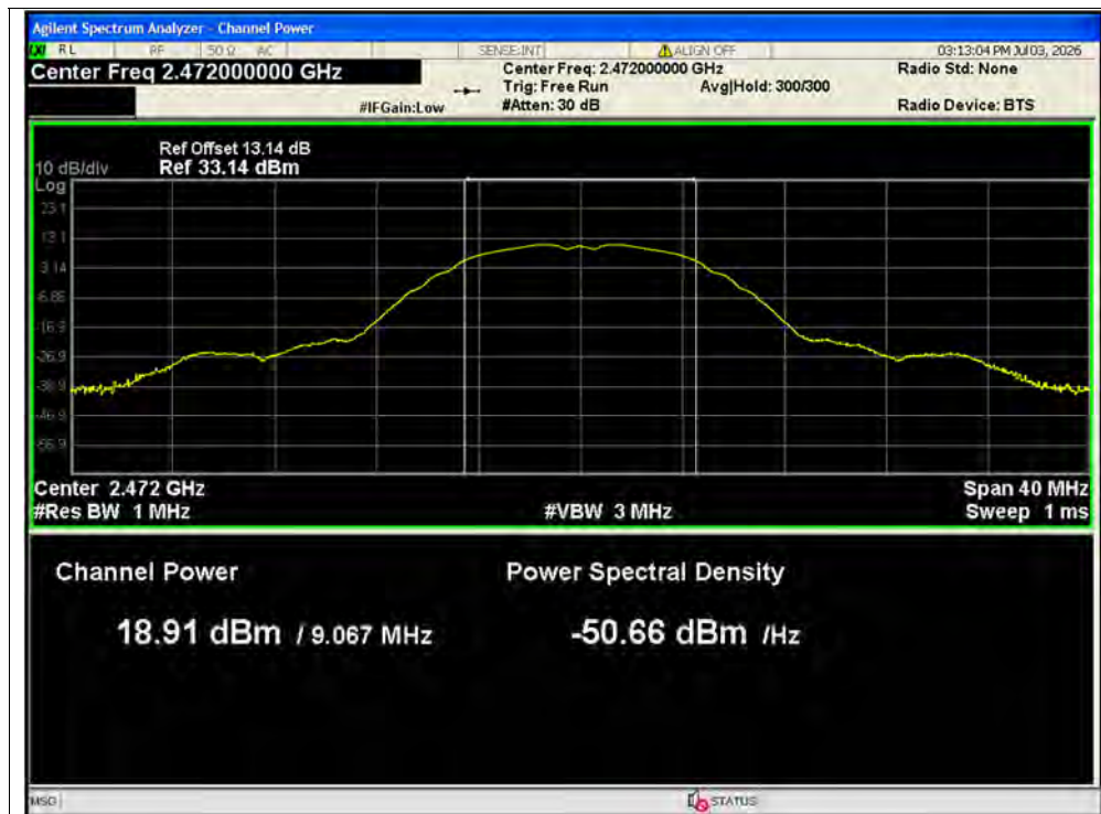
Peak Power NVNT b 2472MHz Ant1
