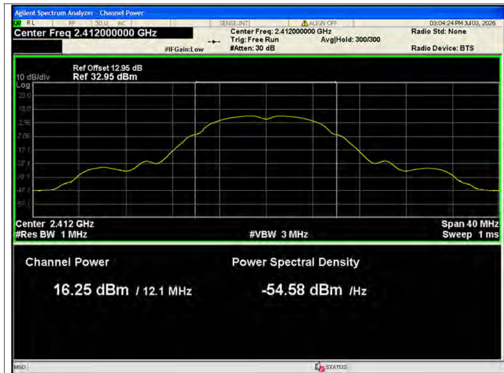
Average Power NVNT b 2412MHz Ant1
