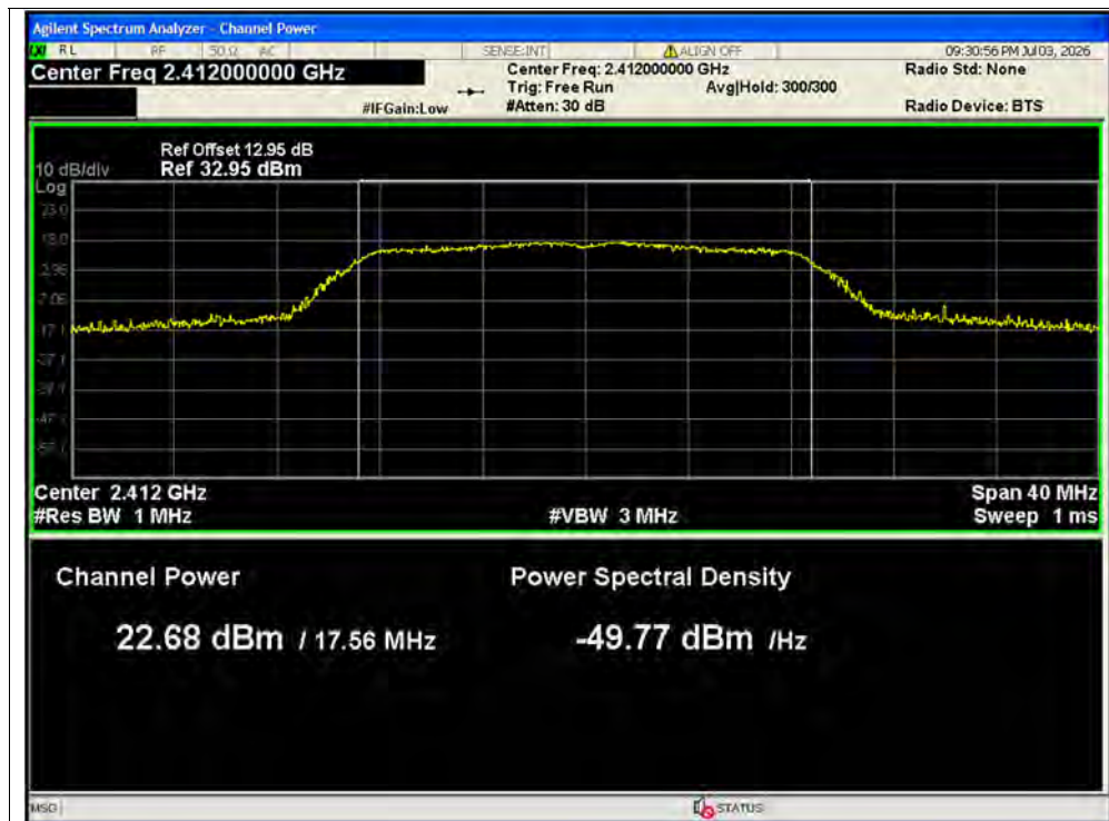
Peak Power NVNT n20 2412MHz Ant1
