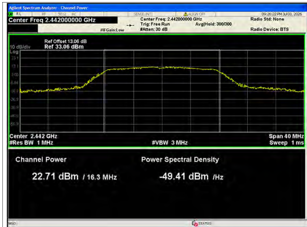
Peak Power NVNT g 2442MHz Ant1
