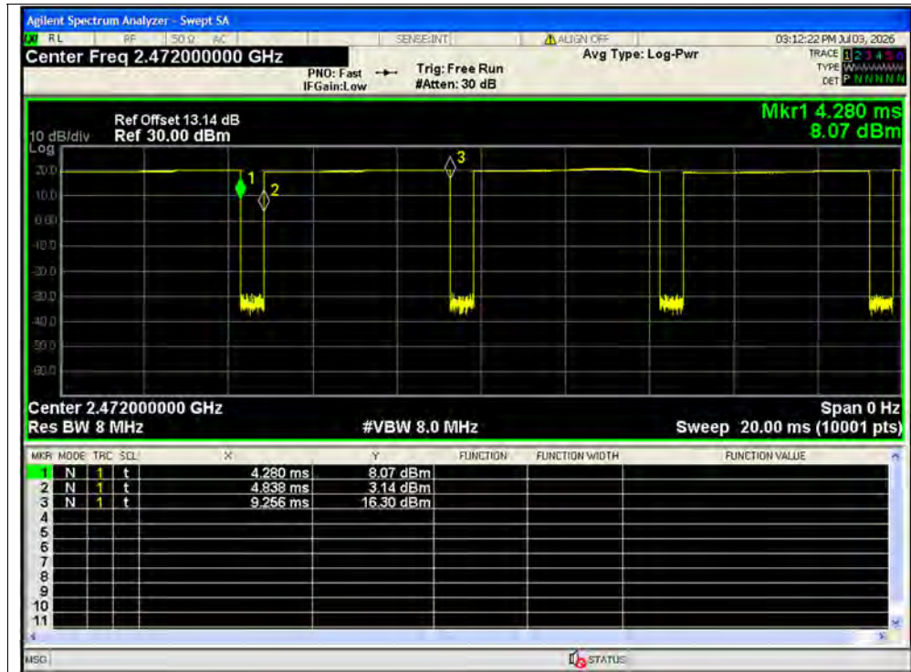
Duty Cycle NVNT b 2472MHz Ant1
