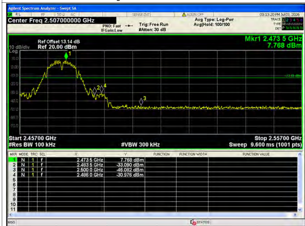
Band Edge NVNT b 2472MHz Ant1 Emission
