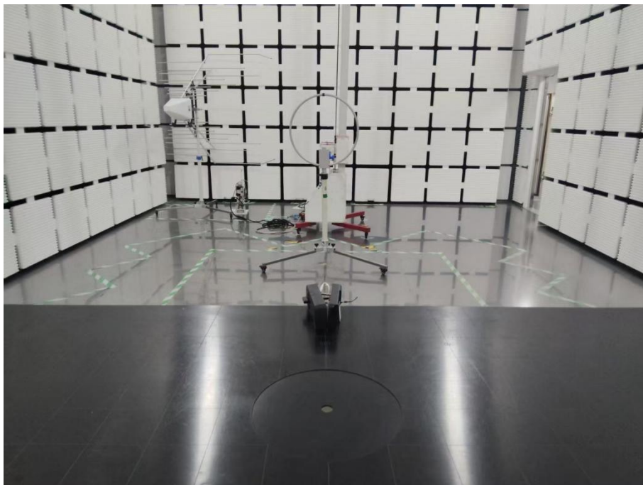
Field Strength of The Fundamental Signal Emissions in frequency bands (below 30MHz)-loop antenna
