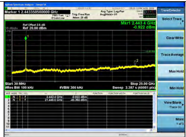
802.11n40 on Channel 09
