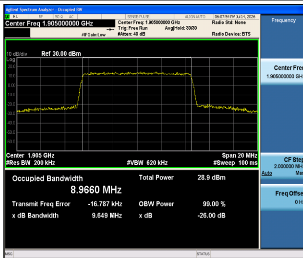
Band2-10MHz-16QAM-19150-50RB#0-PASS
