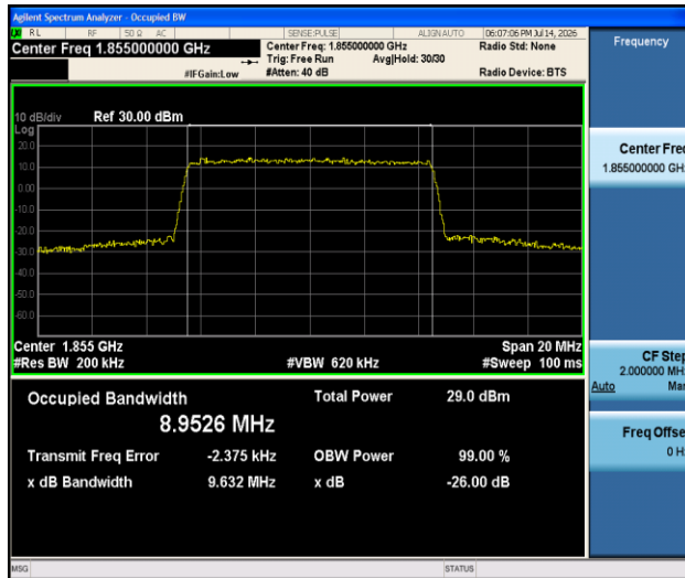
Band2-10MHz-16QAM-18650-50RB#0-PASS
