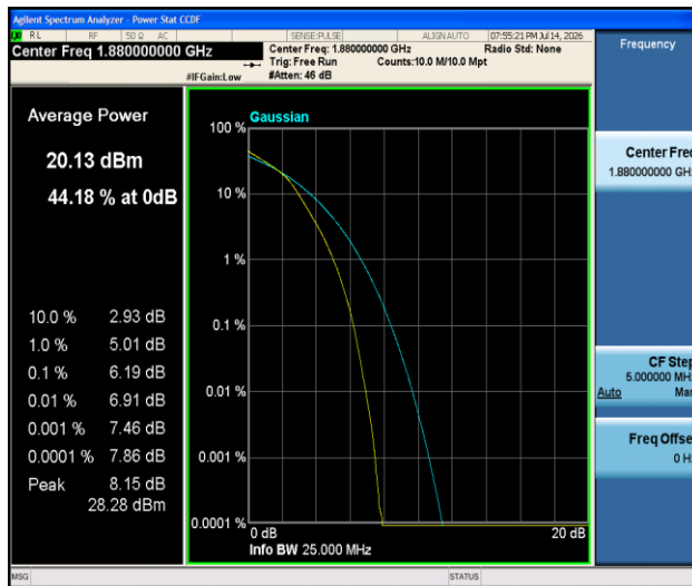
Band2-20MHz-16QAM-18900-100RB#0-PASS
