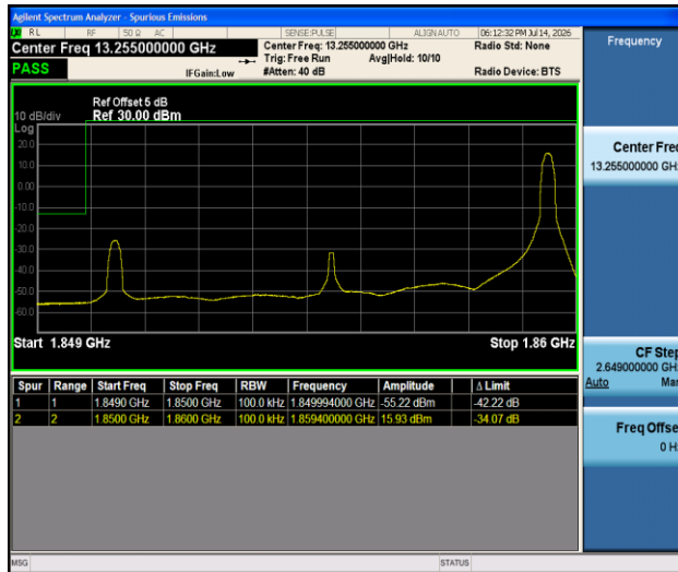
Band2-10MHz-16QAM-18650-1RB#49-PASS
