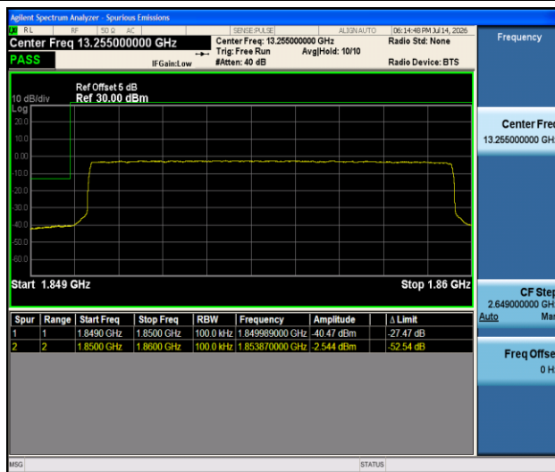
Band2-10MHz-16QAM-18650-50RB#0-PASS
