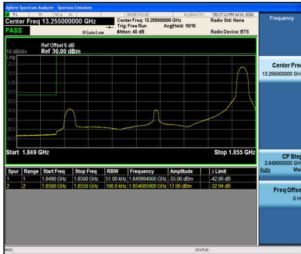
Band2-5MHz-16QAM-18625-1RB#24-PASS
