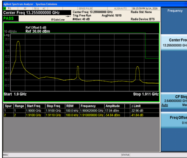
Band2-10MHz-QPSK-19150-1RB#0-PASS
