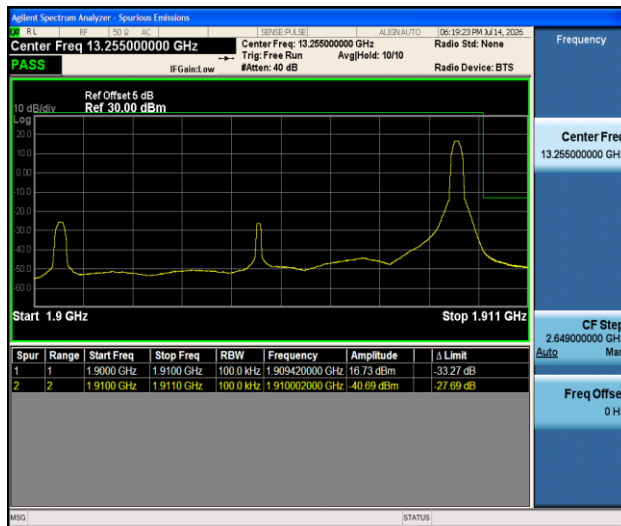
Band2-10MHz-16QAM-19150-1RB#49-PASS
