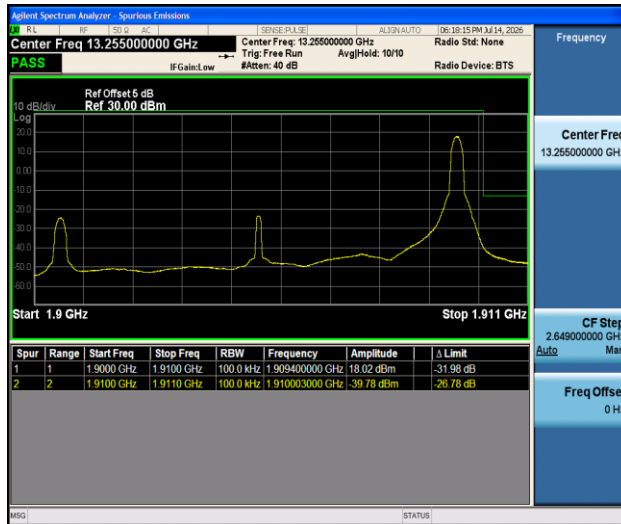
Band2-10MHz-QPSK-19150-1RB#49-PASS
