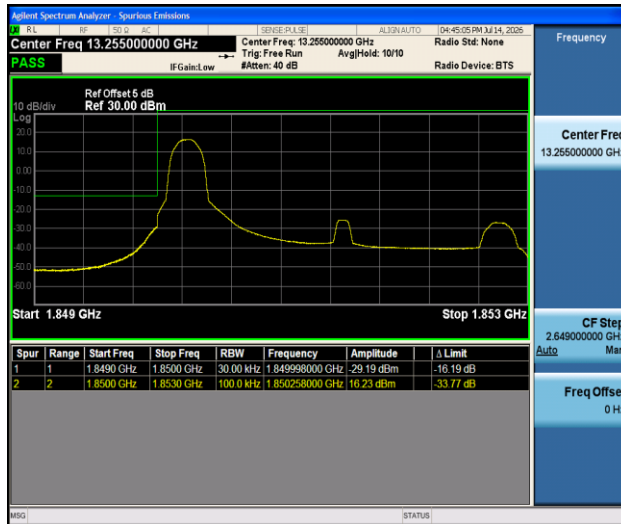
Band2-3MHz-16QAM-18615-1RB#0-PASS
