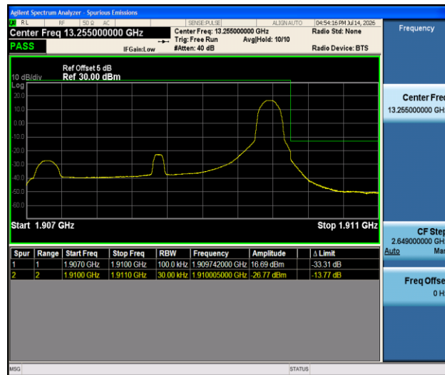
Band2-3MHz-16QAM-19185-1RB#14-PASS
