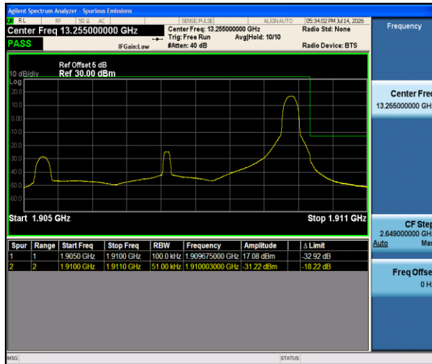
Band2-5MHz-16QAM-19175-1RB#24-PASS
