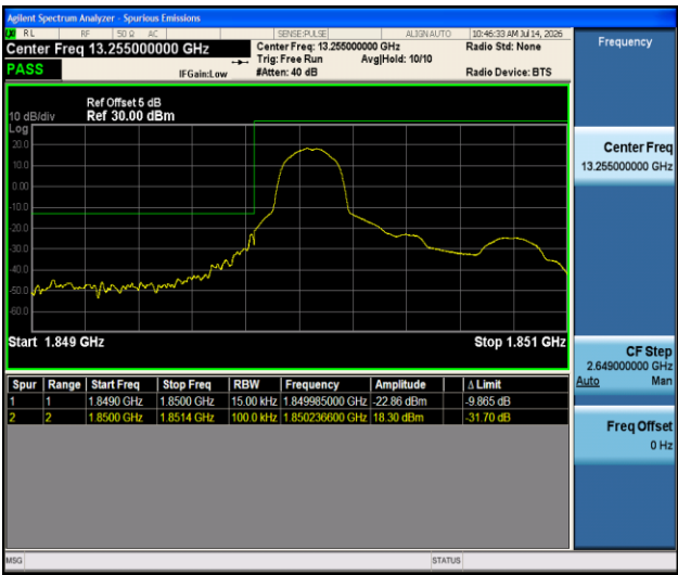
Band2-1.4MHz-QPSK-18607-1RB#0-PASS
