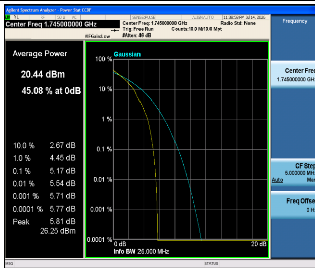
Band4-20MHz-QPSK-20300-1RB#0-PASS
