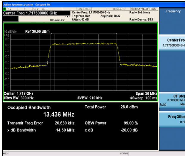
Band4-15MHz-16QAM-20025-75RB#0-PASS
