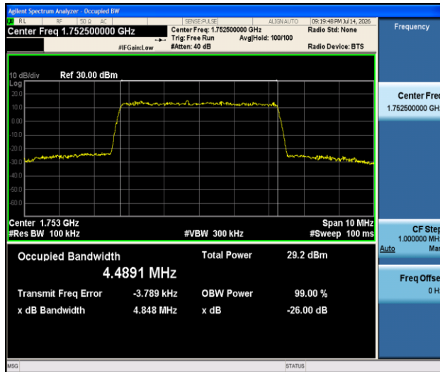
Band4-5MHz-QPSK-20375-25RB#0-PASS
