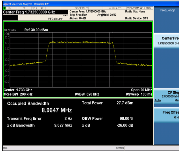
Band4-10MHz-16QAM-20175-50RB#0-PASS
