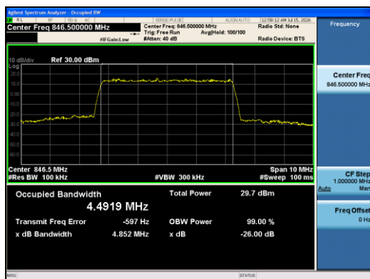
Band5-5MHz-QPSK-20625-25RB#0-PASS
