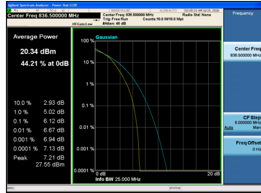
Band5-10MHz-16QAM-20525-50RB#0-PASS
