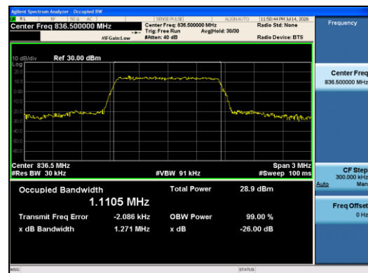
Band5-1.4MHz-16QAM-20525-6RB#0-PASS
