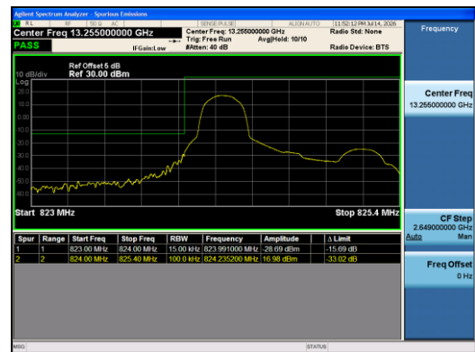
Band5-1.4MHz-16QAM-20407-1RB#0-PASS
