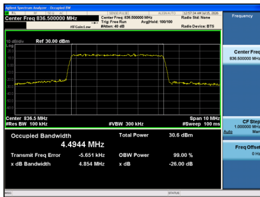
Band5-5MHz-QPSK-20525-25RB#0-PASS
