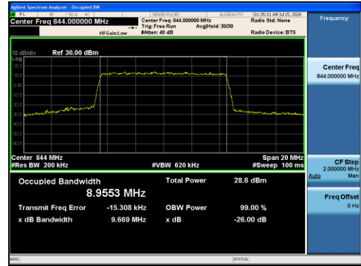
Band5-10MHz-16QAM-20600-50RB#0-PASS
