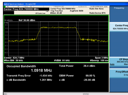
Band5-1.4MHz-16QAM-20407-6RB#0-PASS
