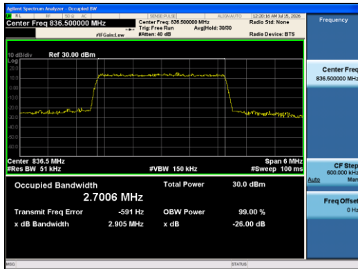
Band5-3MHz-QPSK-20525-15RB#0-PASS
