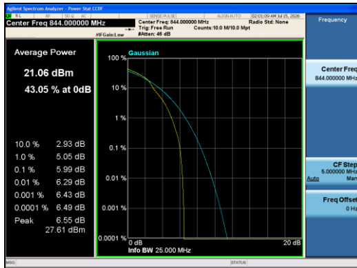
Band5-10MHz-16QAM-20600-1RB#0-PASS
