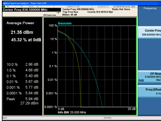
Band5-10MHz-16QAM-20525-1RB#0-PASS
