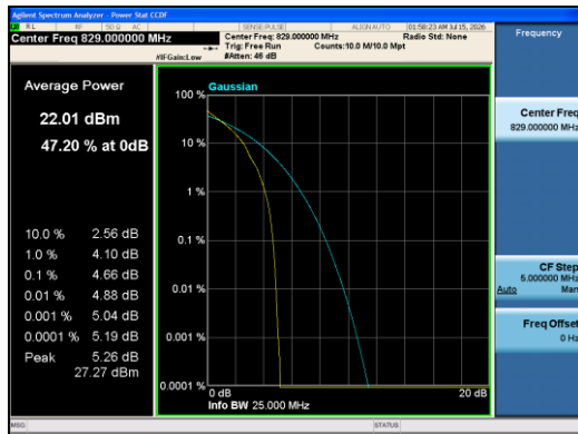
Band5-10MHz-QPSK-20450-1RB#0-PASS
