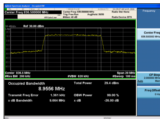
Band5-10MHz-16QAM-20525-50RB#0-PASS
