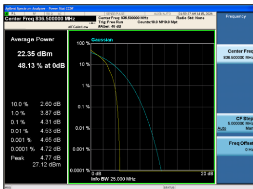
Band5-10MHz-QPSK-20525-1RB#0-PASS
