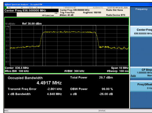
Band5-5MHz-16QAM-20525-25RB#0-PASS
