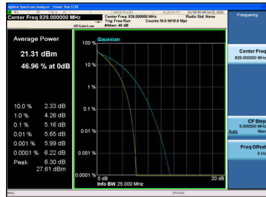
Band5-10MHz-QPSK-20450-50RB#0-PASS
