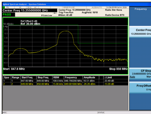
Band5-1.4MHz-16QAM-20643-1RB#5-PASS
