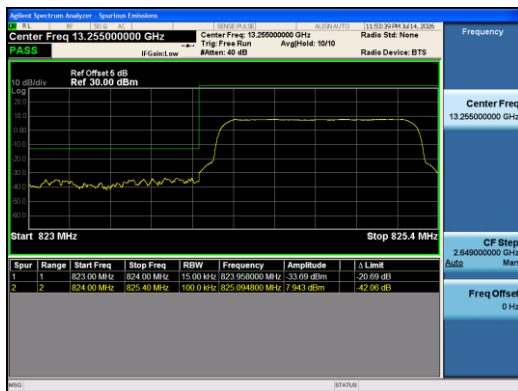
Band5-1.4MHz-QPSK-20407-6RB#0-PASS
