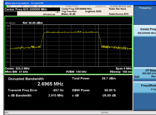
Band5-3MHz-16QAM-20415-15RB#0-PASS
