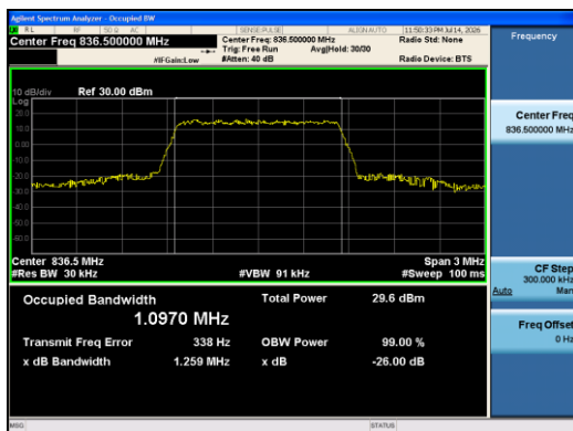
Band5-1.4MHz-QPSK-20525-6RB#0-PASS
