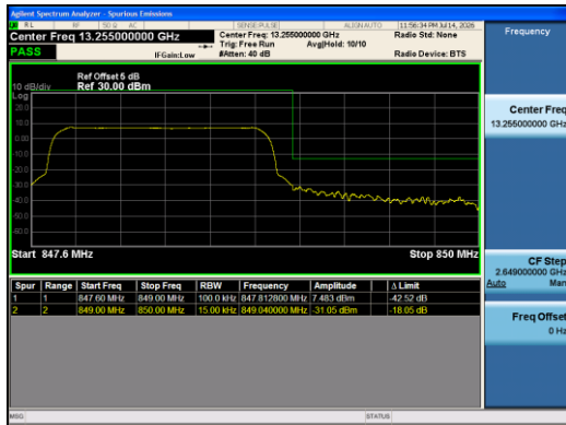
Band5-1.4MHz-QPSK-20643-6RB#0-PASS
