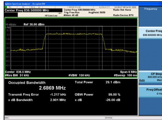
Band5-3MHz-16QAM-20525-15RB#0-PASS
