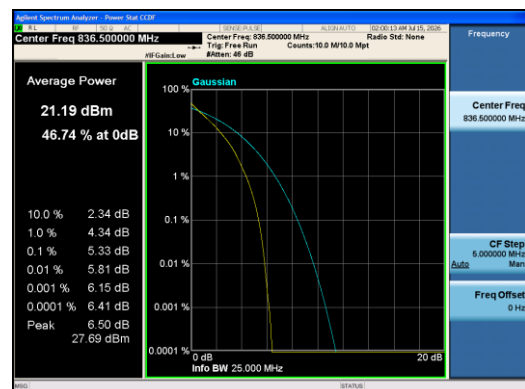
Band5-10MHz-QPSK-20525-50RB#0-PASS
