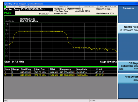
Band5-1.4MHz-16QAM-20643-6RB#0-PASS
