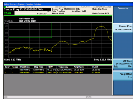
Band5-1.4MHz-QPSK-20407-1RB#5-PASS
