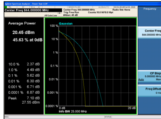
Band5-10MHz-QPSK-20600-50RB#0-PASS
