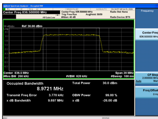
Band5-10MHz-QPSK-20525-50RB#0-PASS
