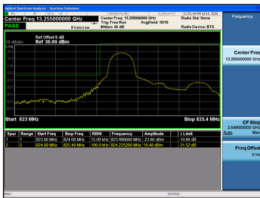
Band5-1.4MHz-QPSK-20407-1RB#0-PASS
