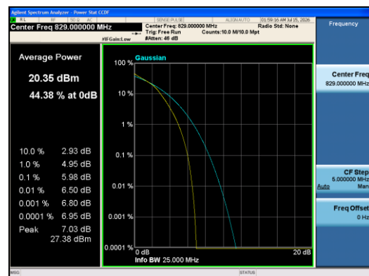
Band5-10MHz-16QAM-20450-50RB#0-PASS
