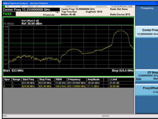
Band5-1.4MHz-16QAM-20407-1RB#5-PASS
