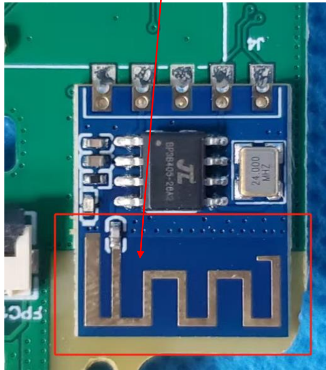
View of wireless antenna
