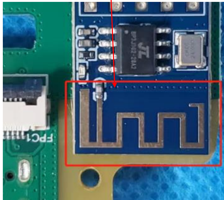
View of wireless antenna
