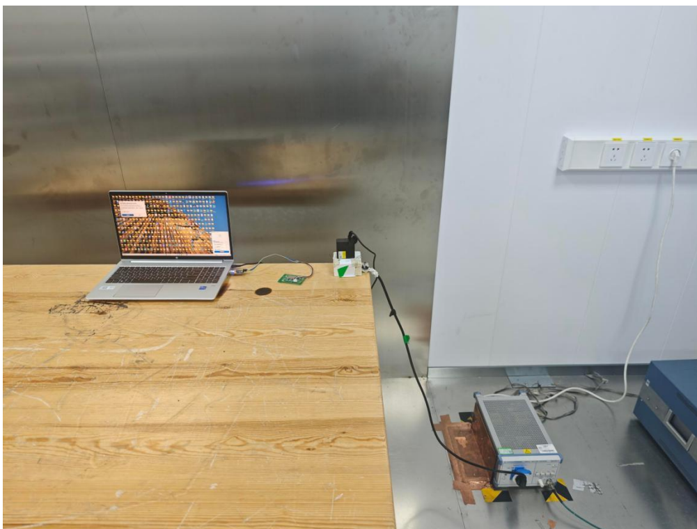
Radiated Emission Test View(9KHz-30MHz)
