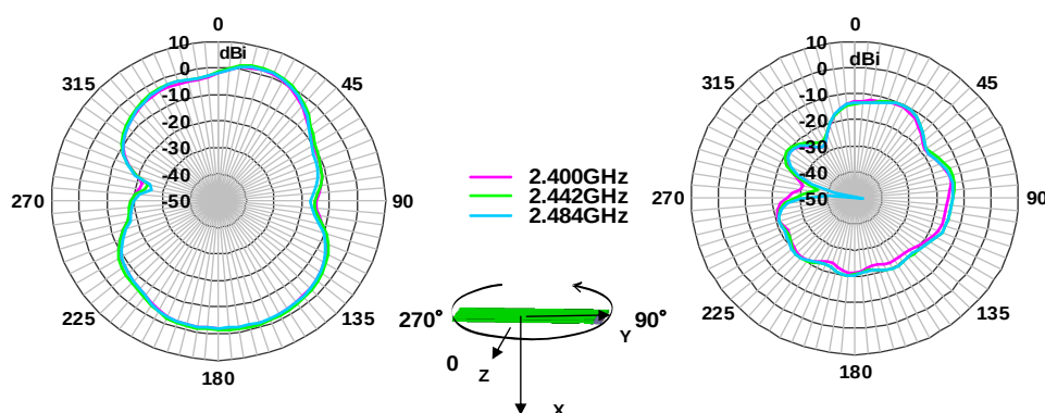
Horizontal Polarization
