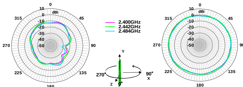
Horizontal Polarization
