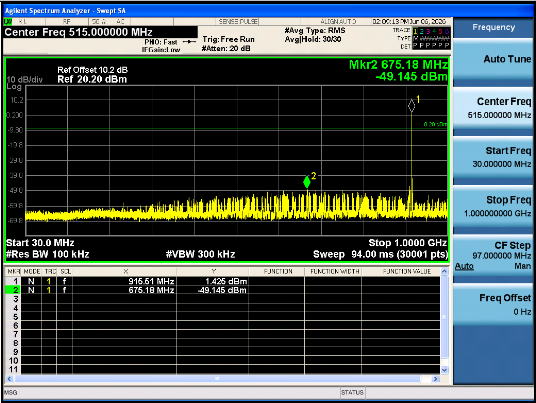
LORA_OFDM_LR-Ant1-915-30~1000-PASS
