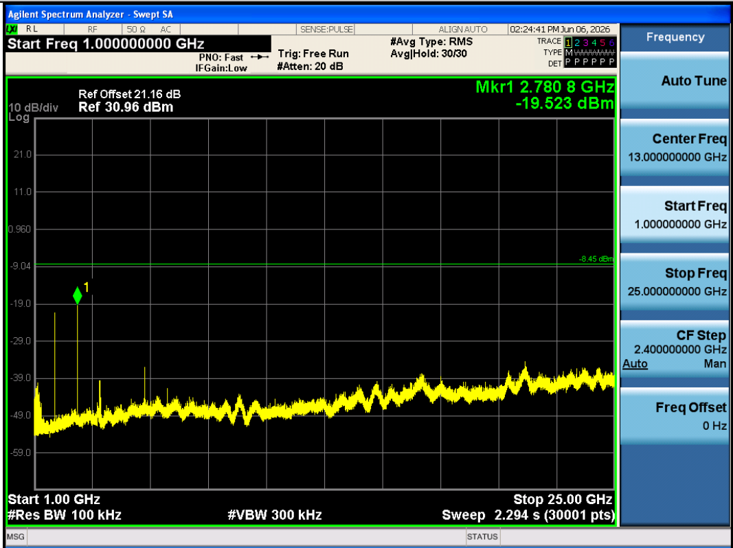
LORA_OFDM_LR-Ant1-927-1000~25000-PASS
