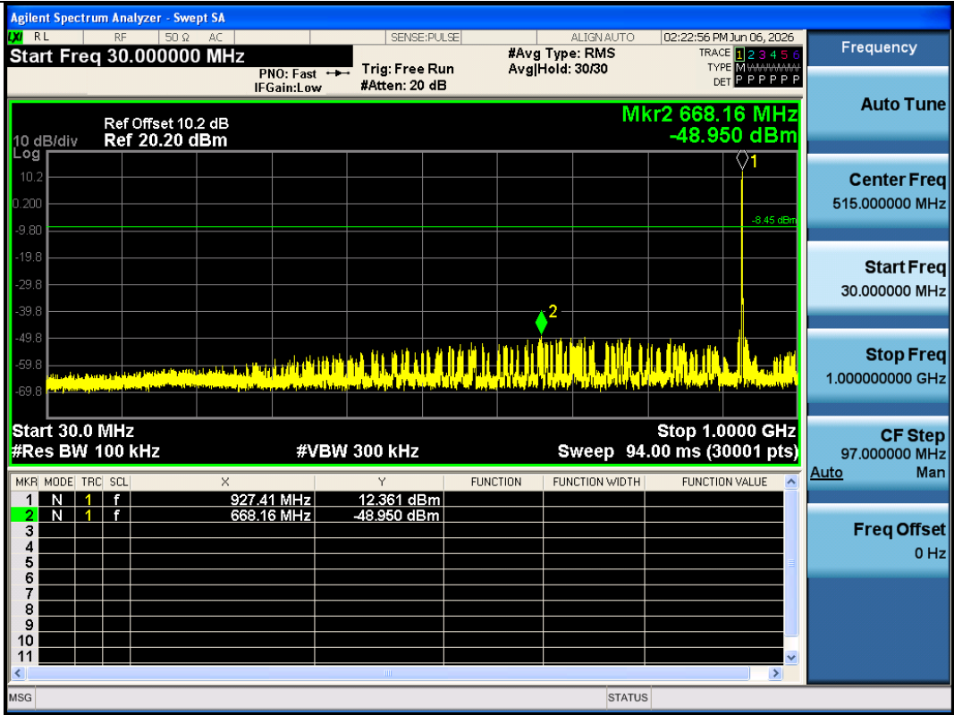
LORA_OFDM_LR-Ant1-927-30~1000-PASS
