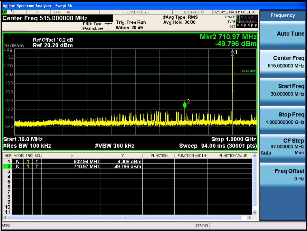
LORA_OFDM_LR-Ant1-903-30~1000-PASS
