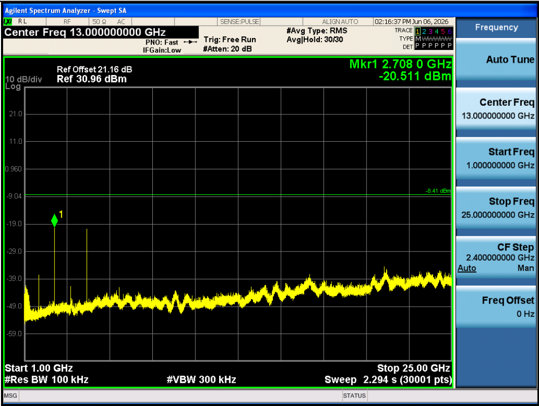
LORA_OFDM_LR-Ant1-903-1000~25000-PASS
