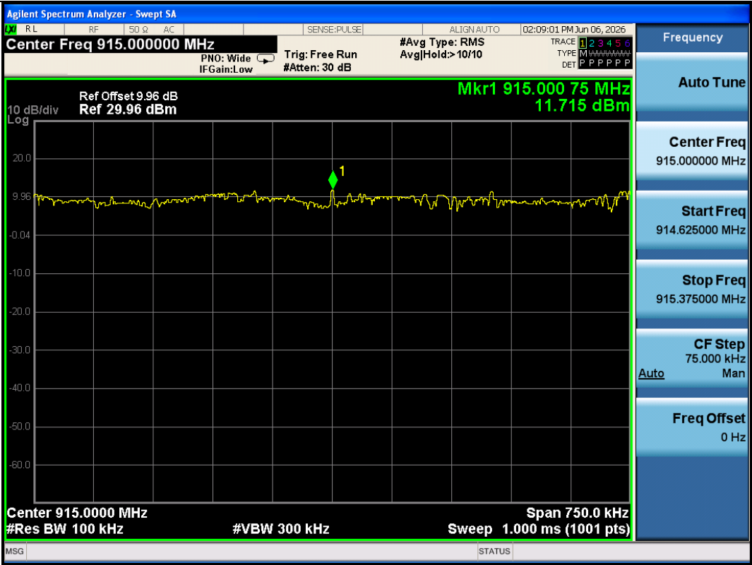
LORA_OFDM_LR-Ant1-915-0~Reference-PASS
