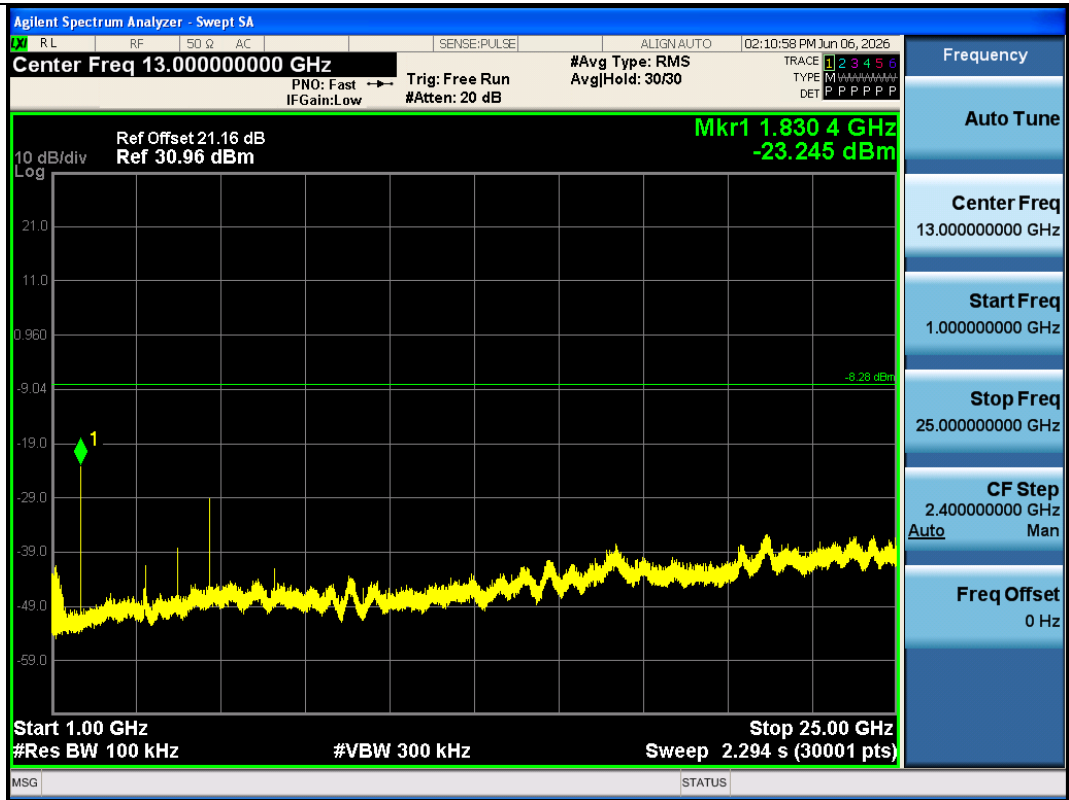
LORA_OFDM_LR-Ant1-915-1000~25000-PASS
