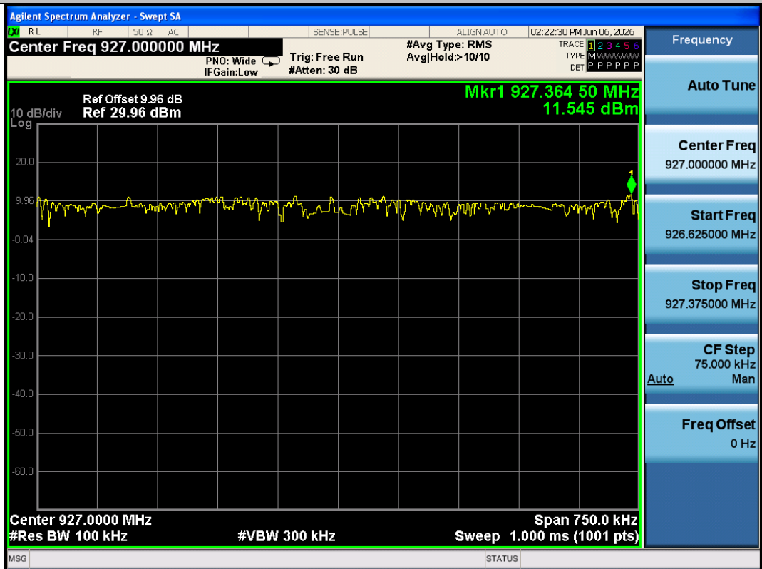
LORA_OFDM_LR-Ant1-927-0~Reference-PASS
