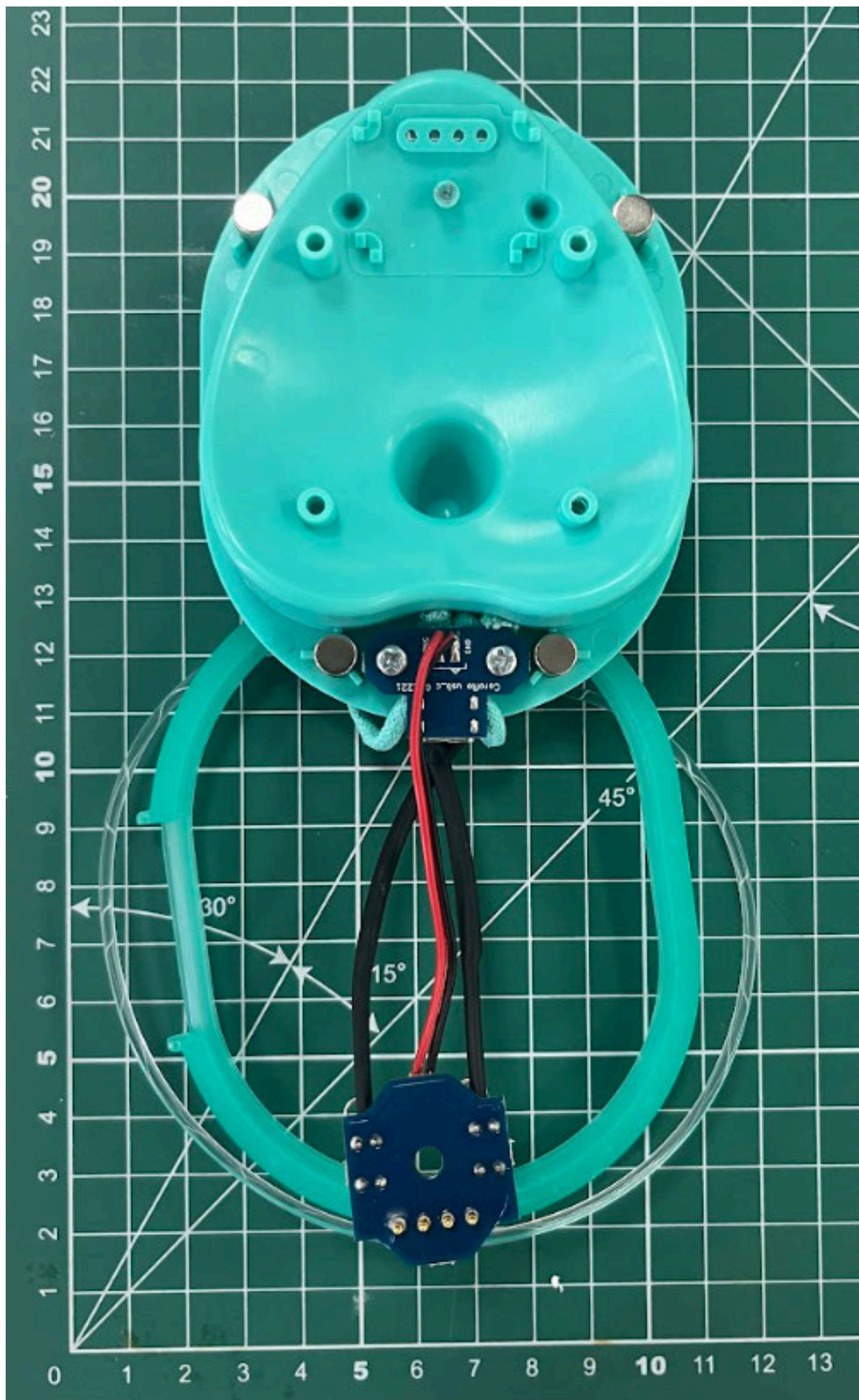
Charging case - Internal components Top
