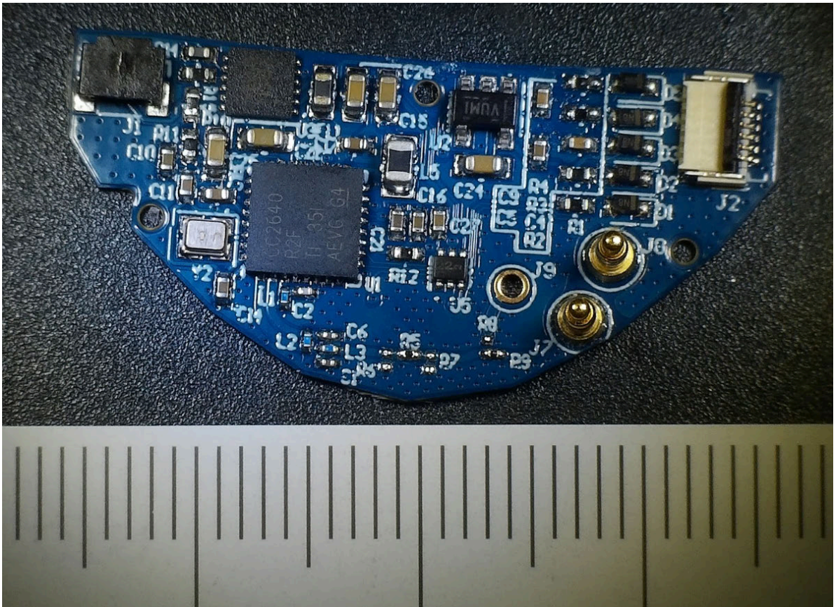
Device - PCB - Top
