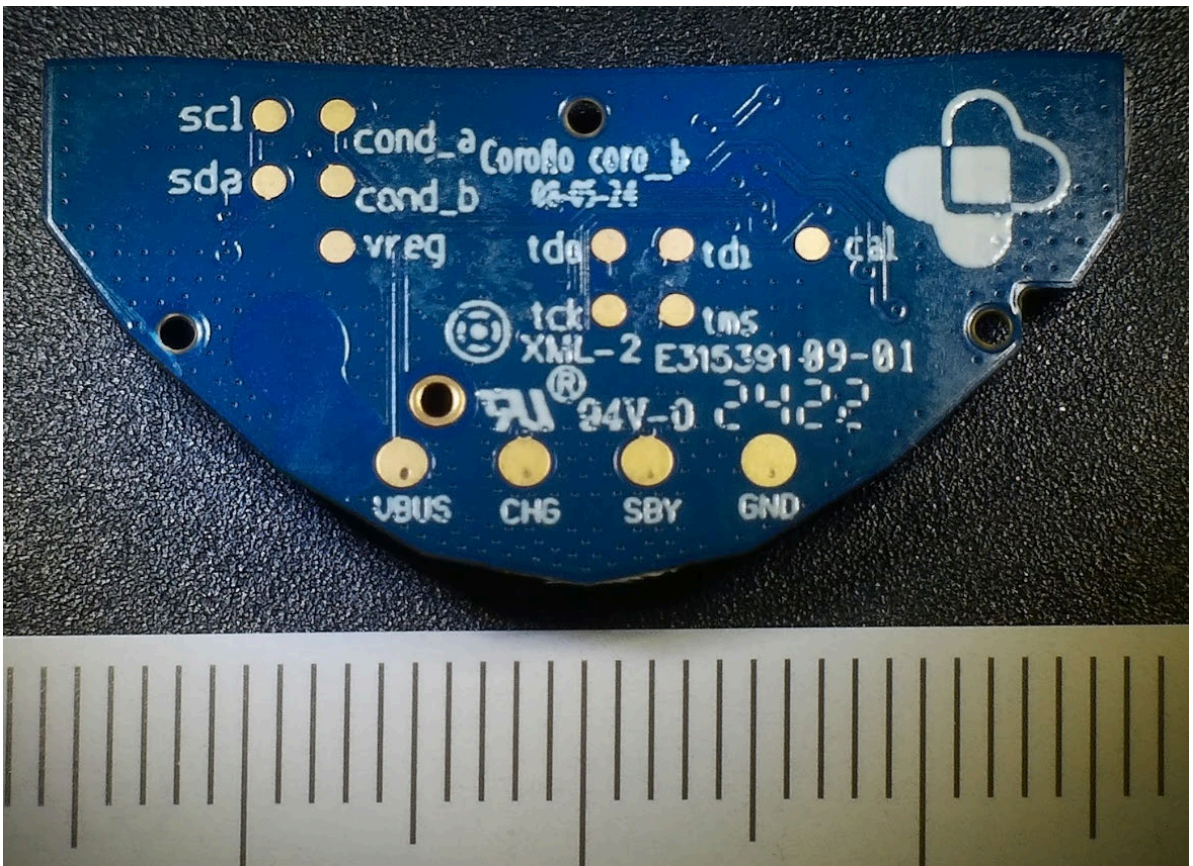
Device - PCB - Bottom
