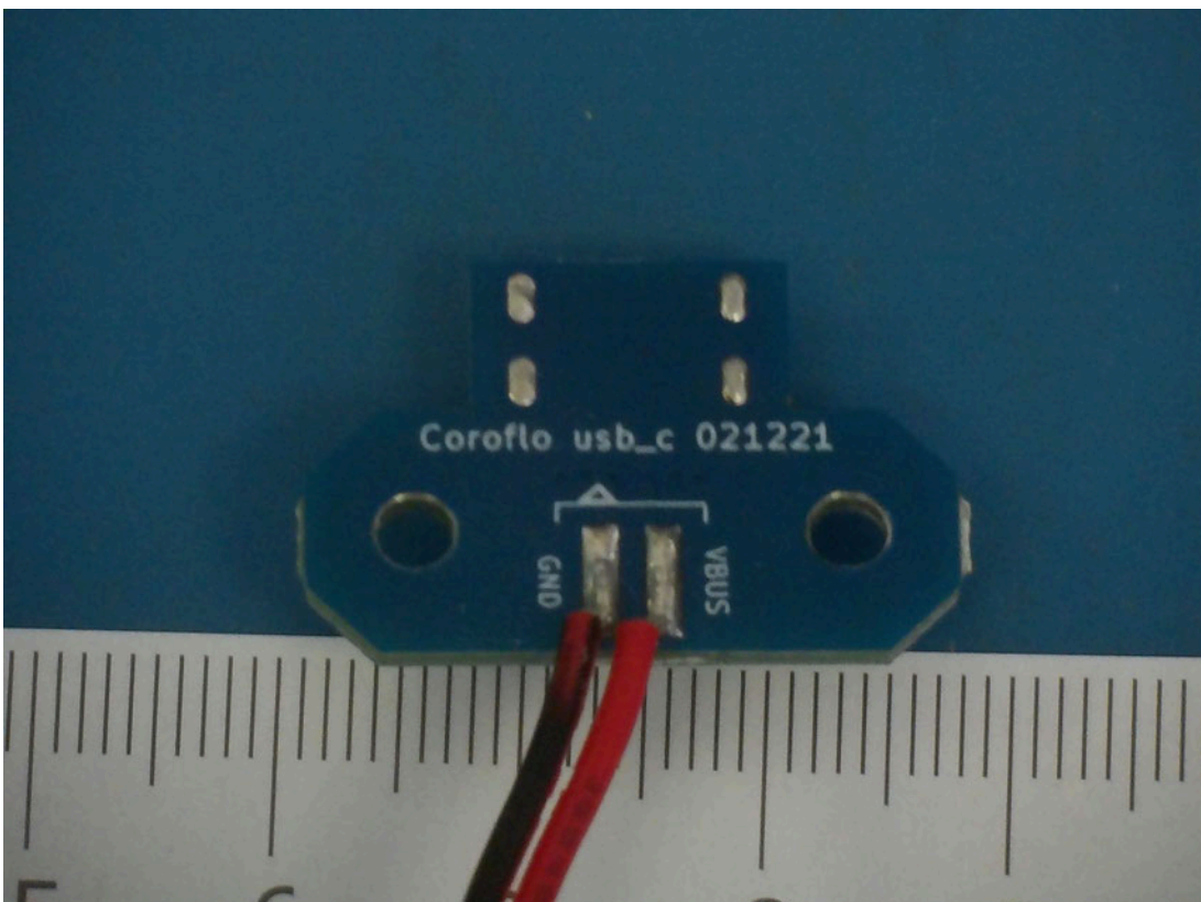
Charging case - USB C Top
