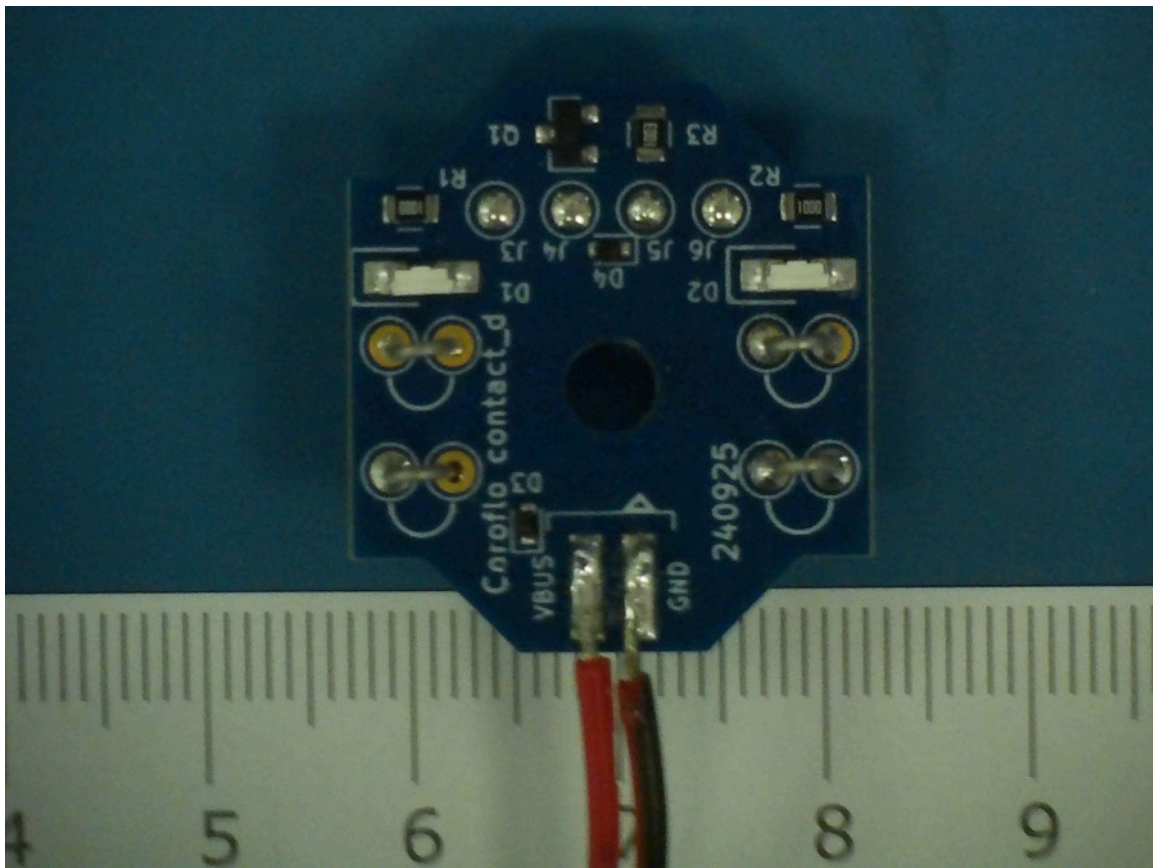
Charging case - Contact_d Top
