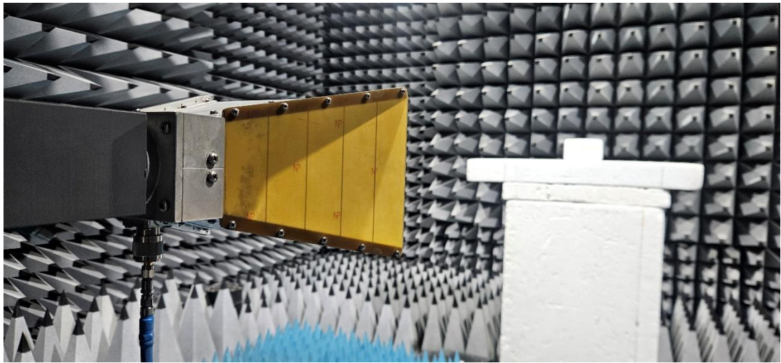
Radiated emissions 1GHz -18GHz
