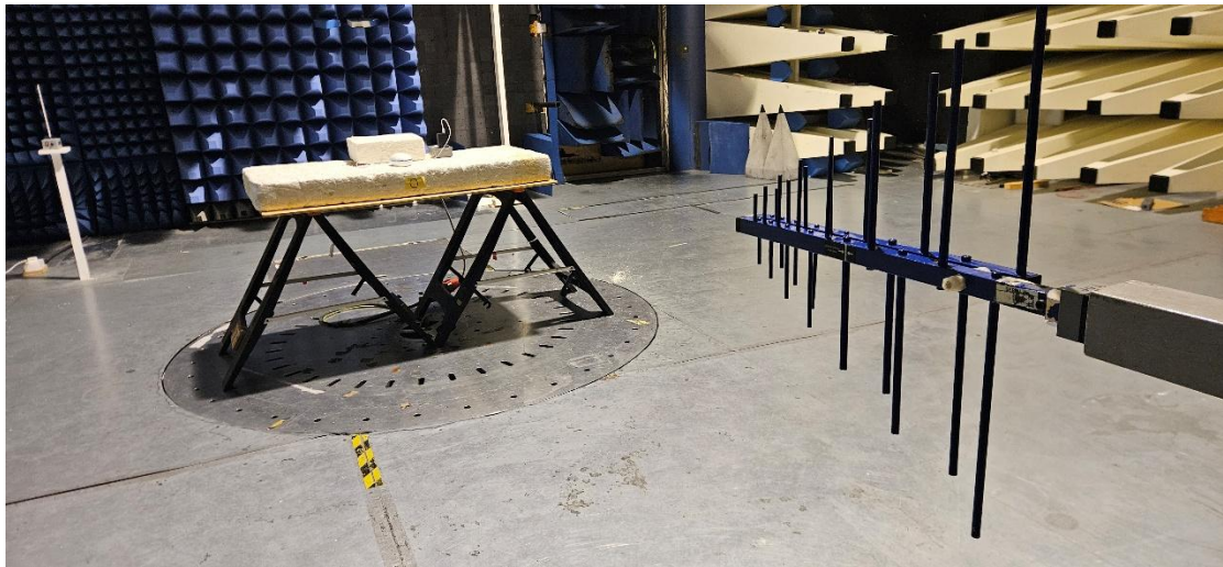
Radiated emissions 300MHz -1GHz
