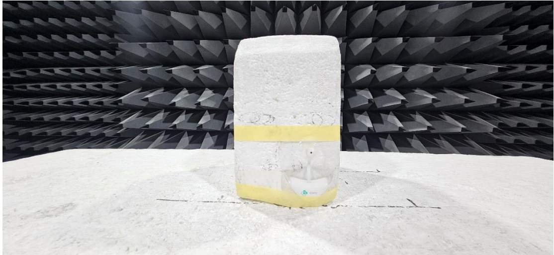
EUT close up radiated emissions
