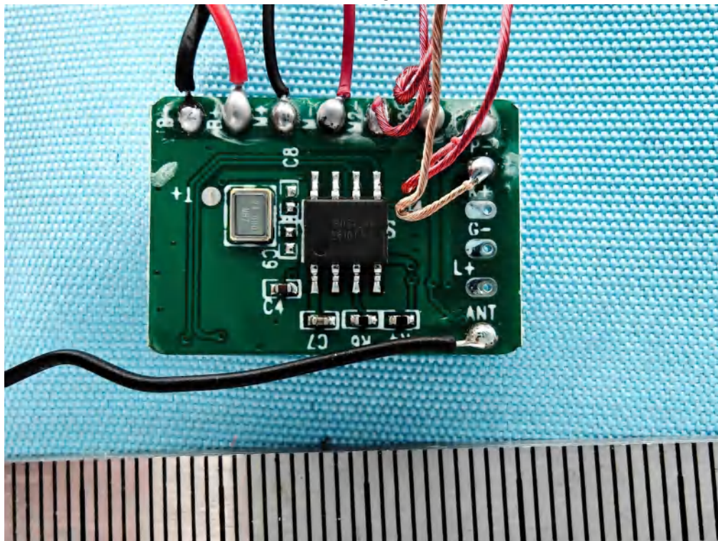
Photo 33 Internal photos of EUT H248
