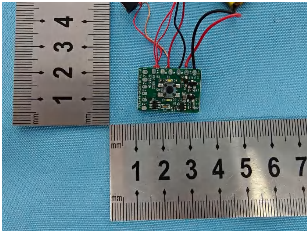
Photo 31 Internal photos of EUT H248
