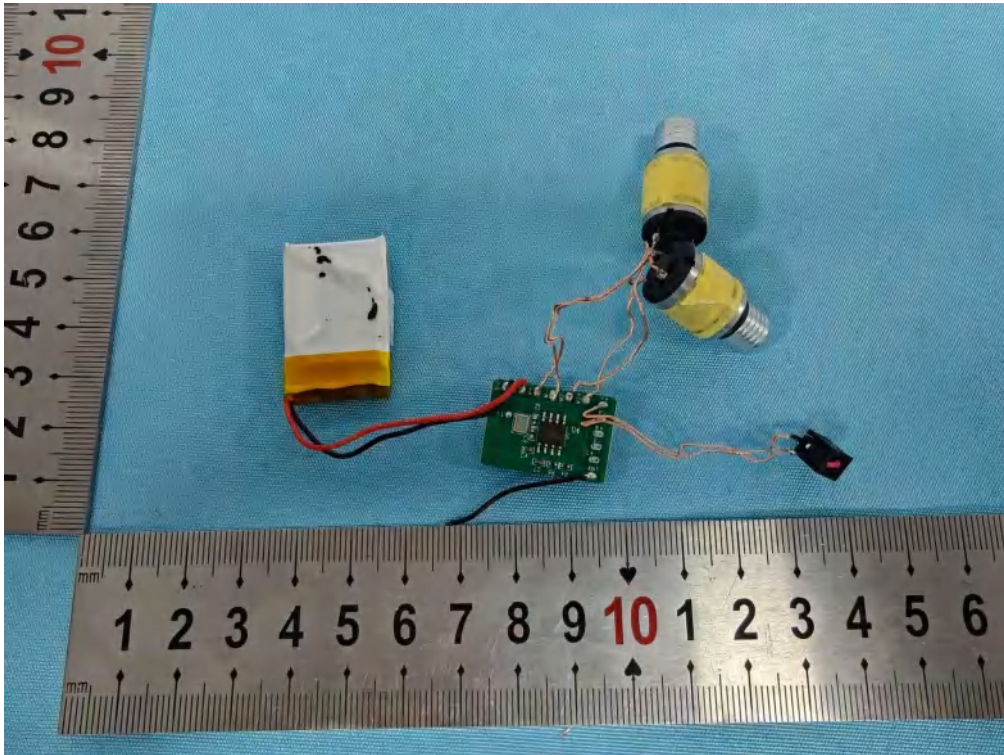
Photo 16 Internal photos of EUT H238
