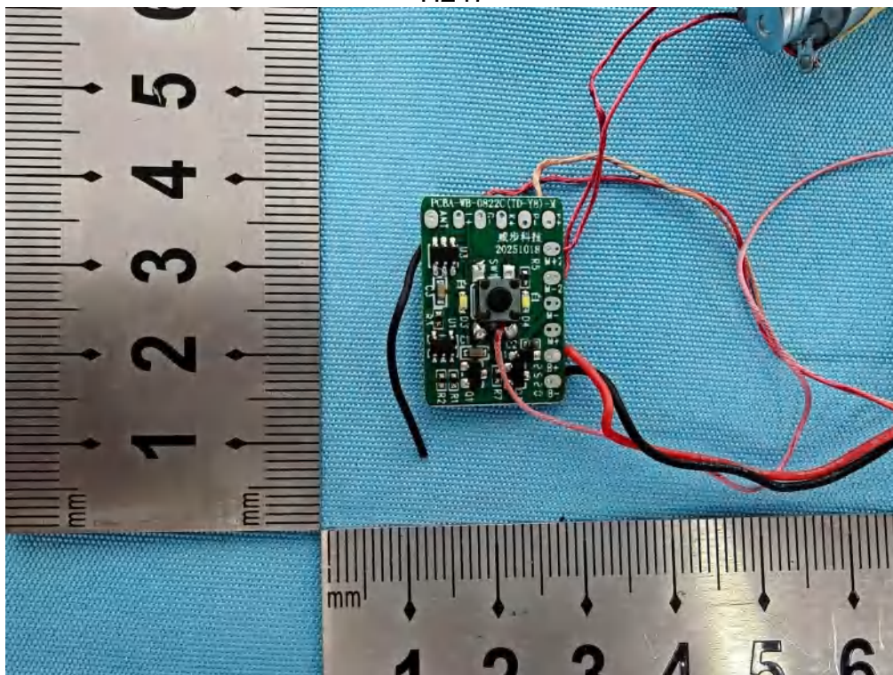
Photo 24 Internal photos of EUT H247
