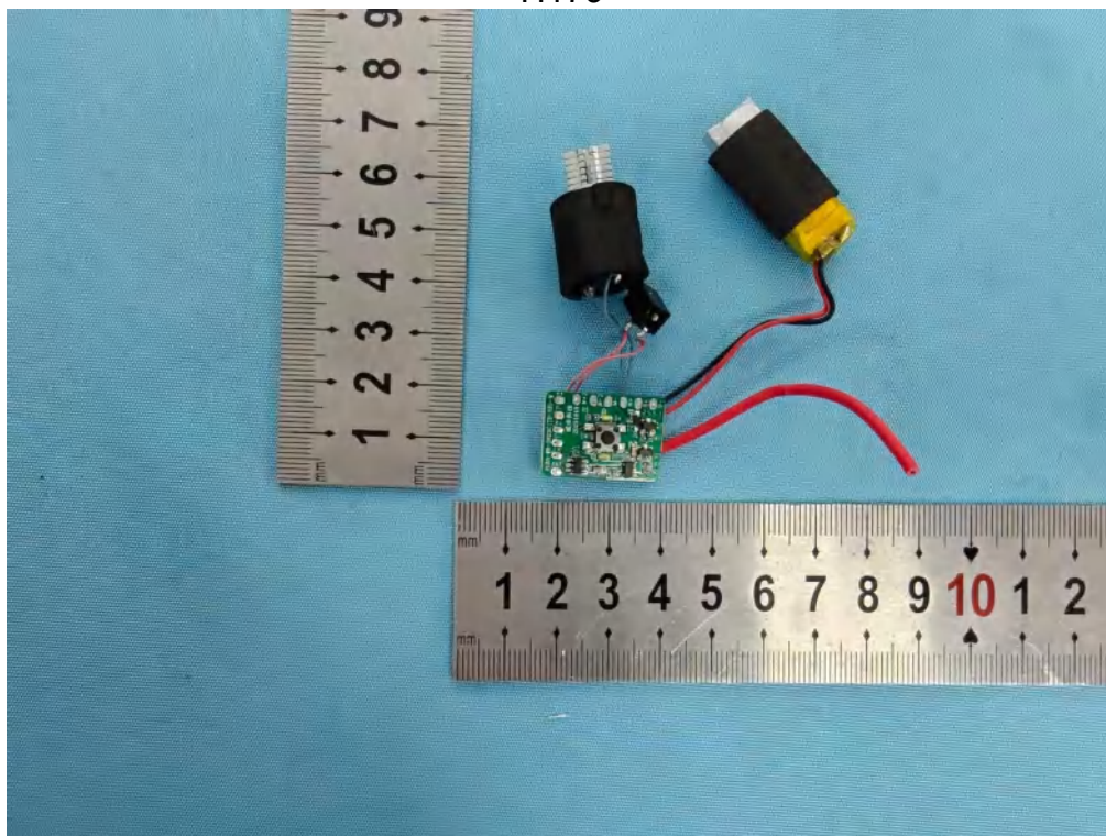
Photo 5 Internal photos of EUT H179
