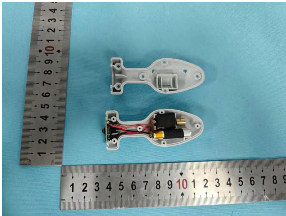
Photo 7 Internal photos of EUT H103
