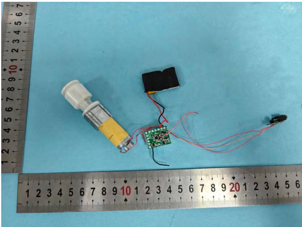
Photo 22 Internal photos of EUT H247
