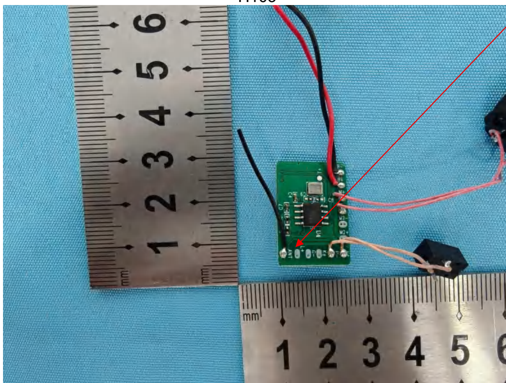
Photo 10 Internal photos of EUT H103
