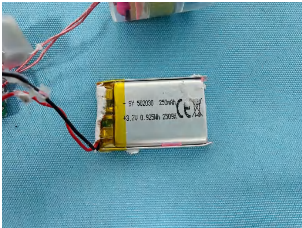
Photo 13 Internal photos of EUT H103
