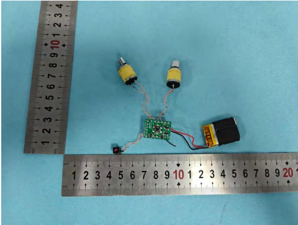
Photo 15 Internal photos of EUT H238
