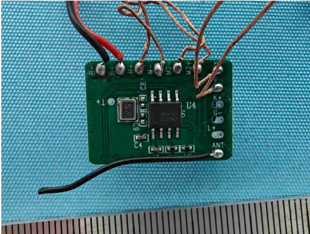
Photo 20 Internal photos of EUT
