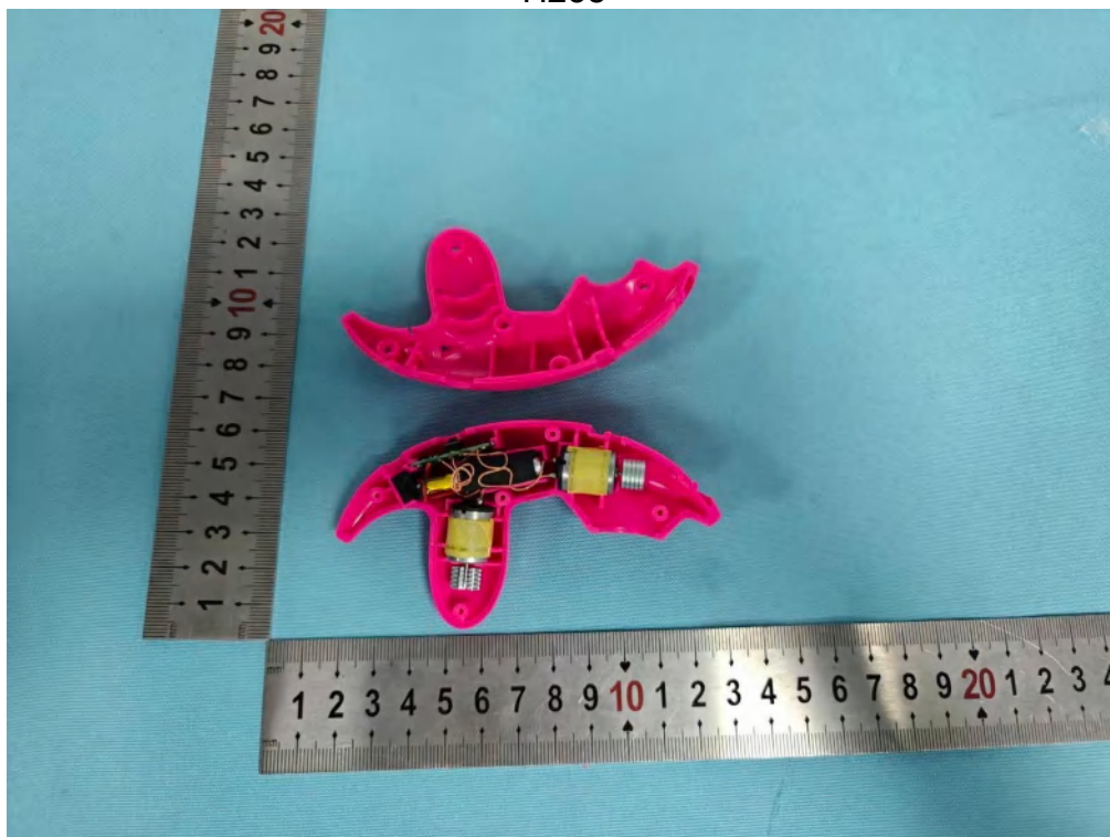
Photo 14 Internal photos of EUT H238
