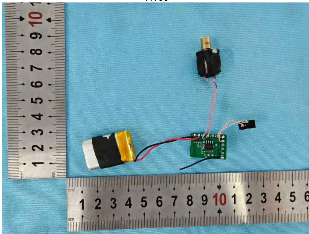
Photo 9 Internal photos of EUT H103
