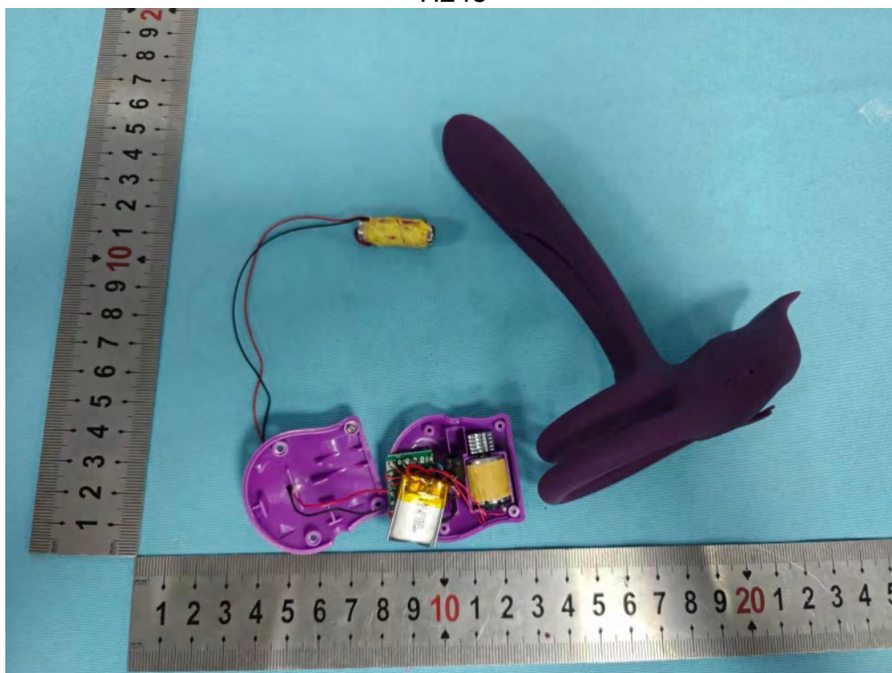
Photo 28 Internal photos of EUT H248
