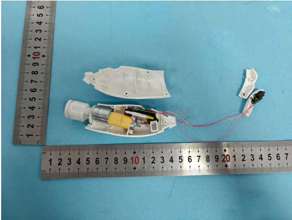
Photo 21 Internal photos of EUT H247
