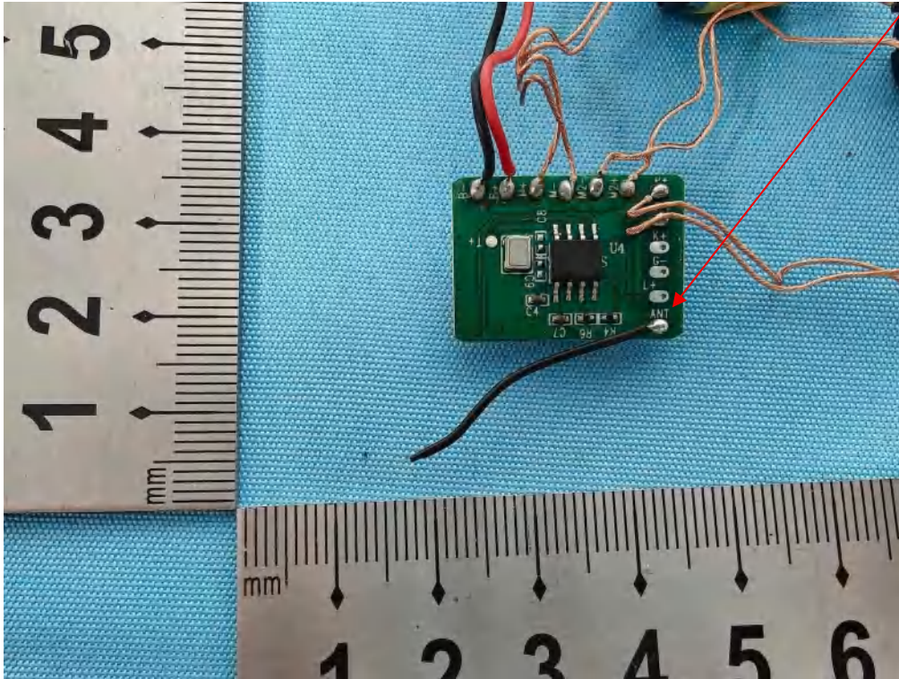
Photo 17 Internal photos of EUT H238
