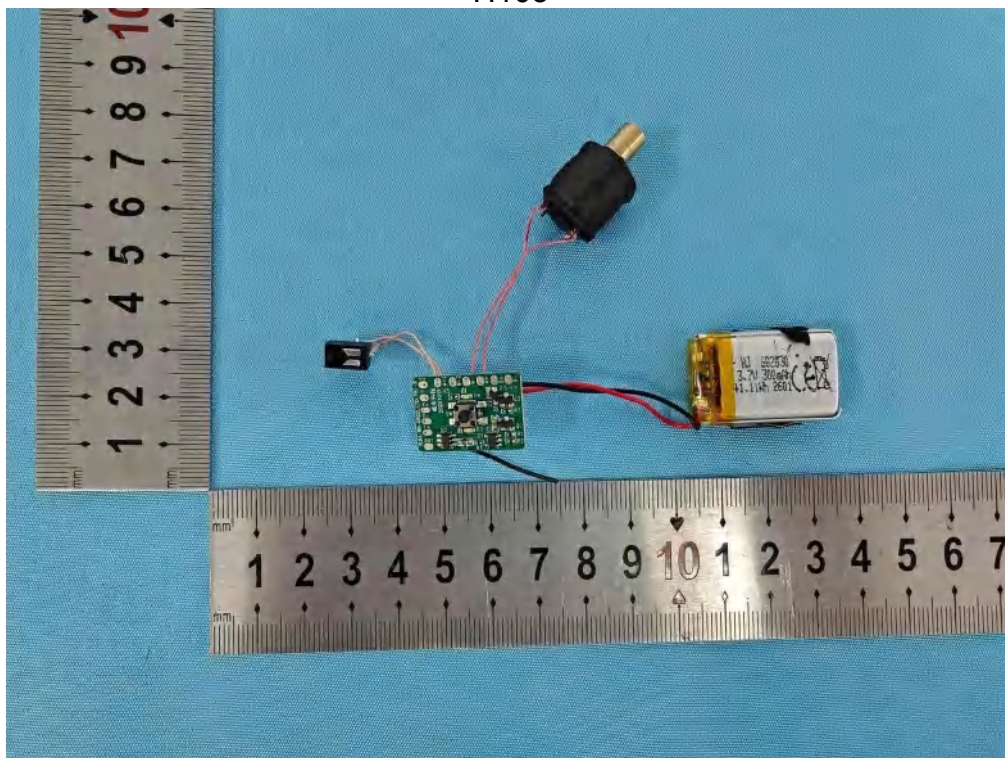
Photo 8 Internal photos of EUT H103
