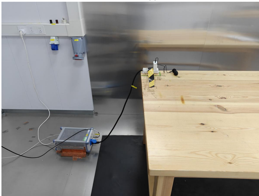
Photo 8 Test Setup Photos of Radiated Emission Test (30-1000MHz)
