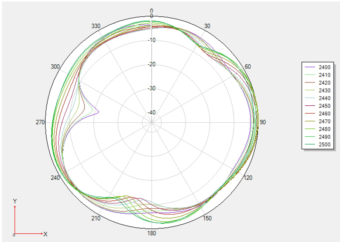
E3 directional diagram
